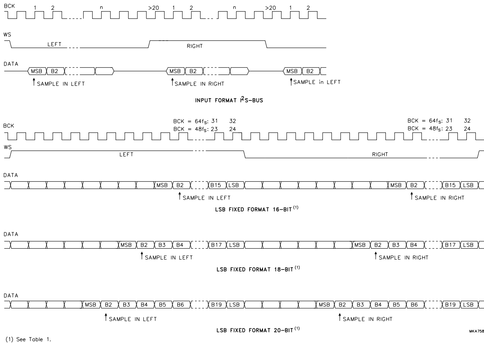
Fig.3 Input formats.
