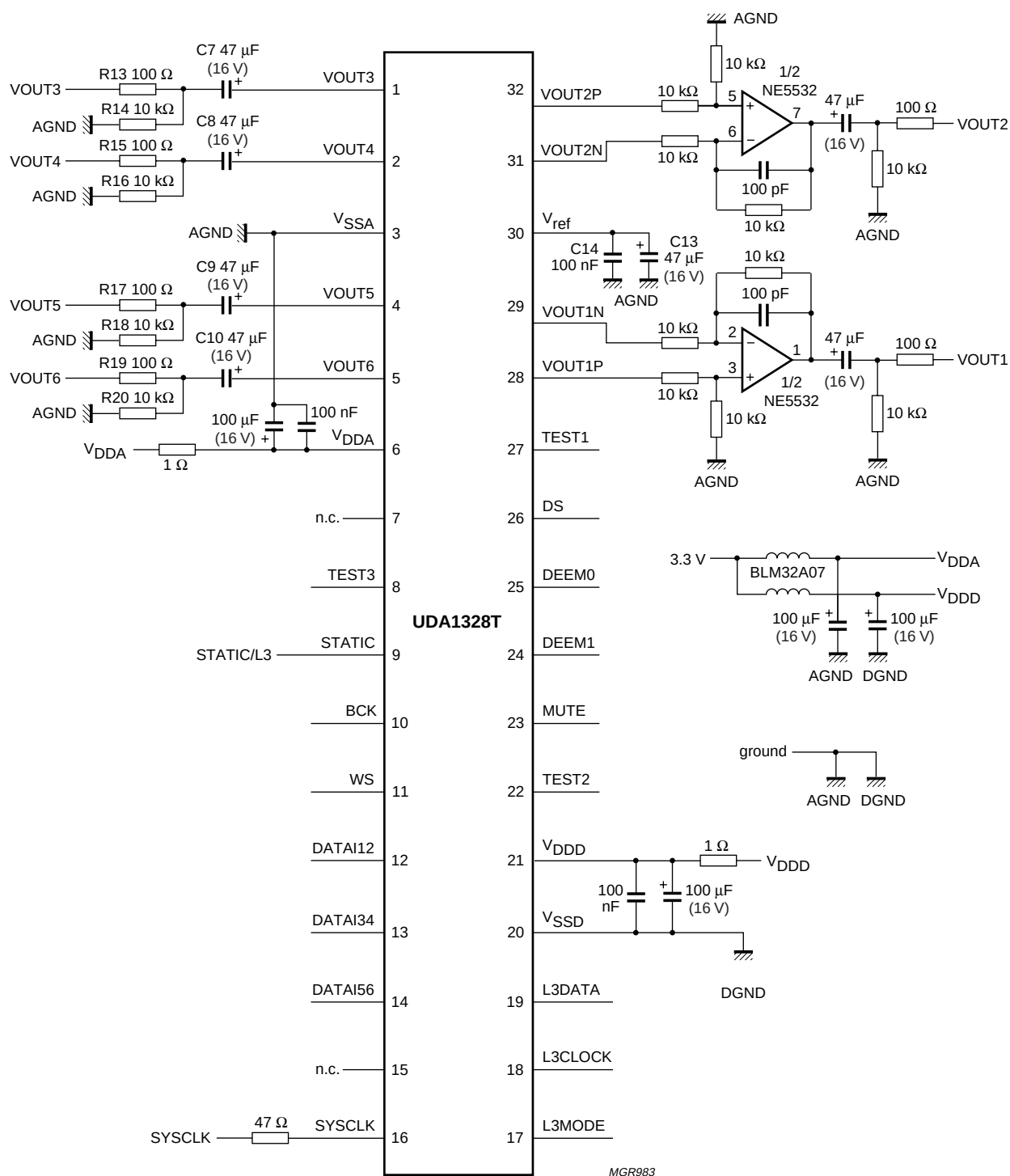
Fig.11 Application diagram.
