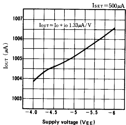
Output current vs. Supply voltage ( V_{\text{EE}} )
