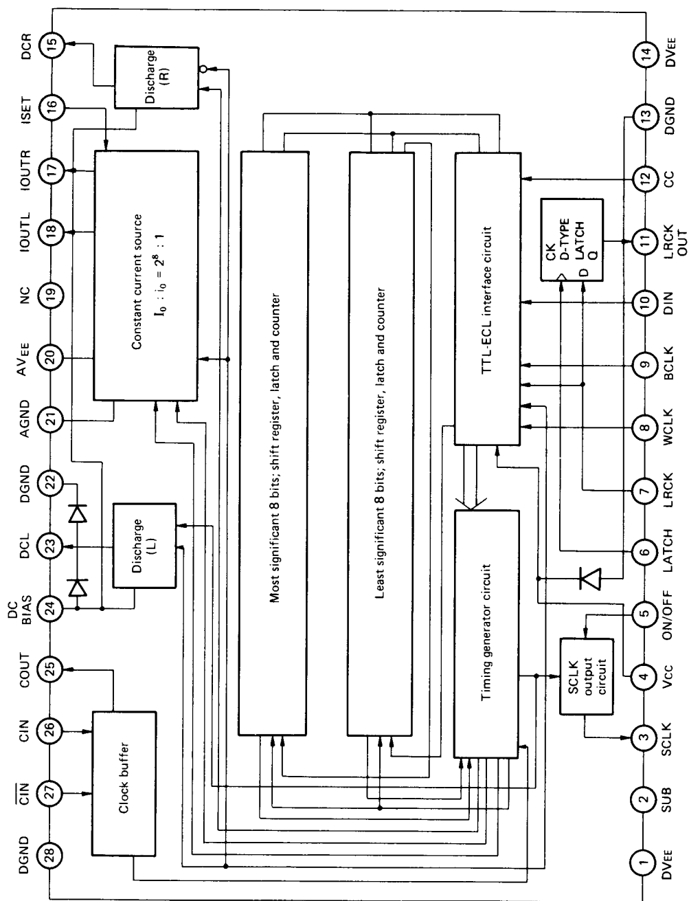
Block Diagram
