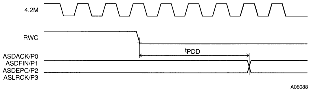
Figure 5 General-Purpose Port Output Timing
