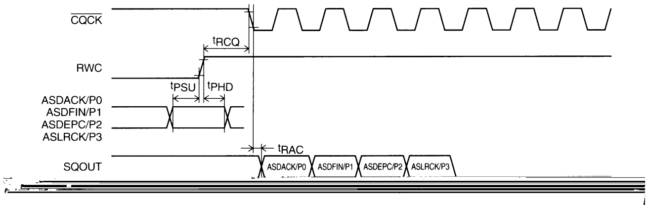
Figure 4 General-Purpose Port Input Timing
