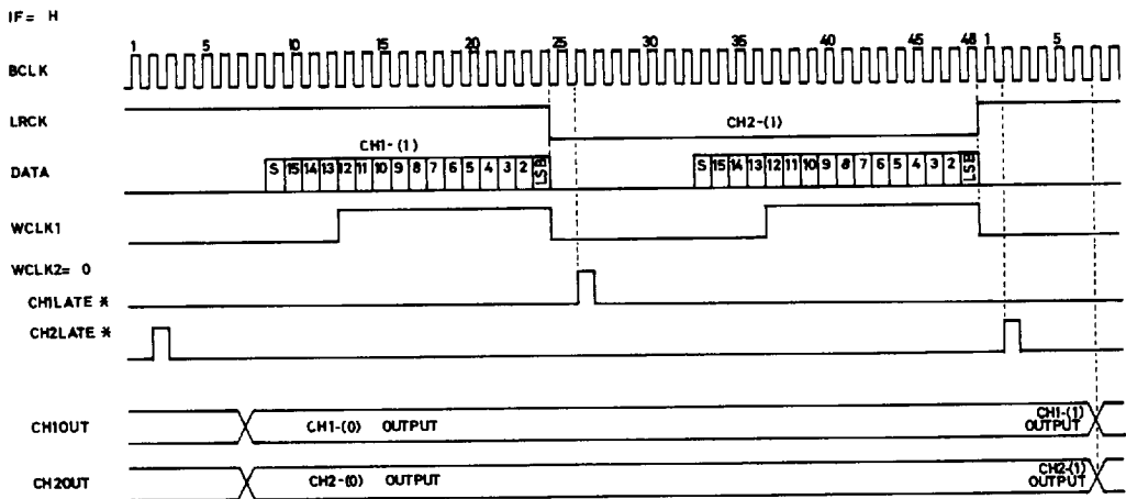
Timing Chart 1
