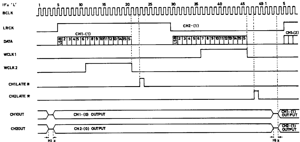
Timing Chart 2
