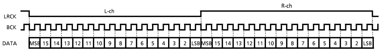
Fig.2a Example of input timing diagram ( L/\overline{R} = "L" )
