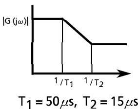
Fig.5 Filter characteristic
