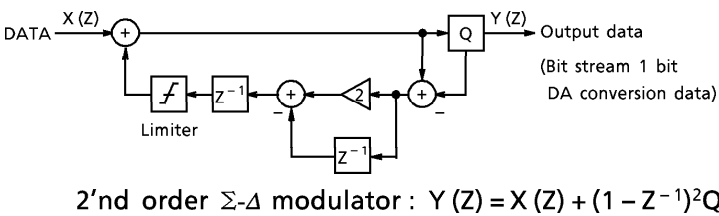
Fig.6 Construction of \Sigma - \Delta modulation DA converter
