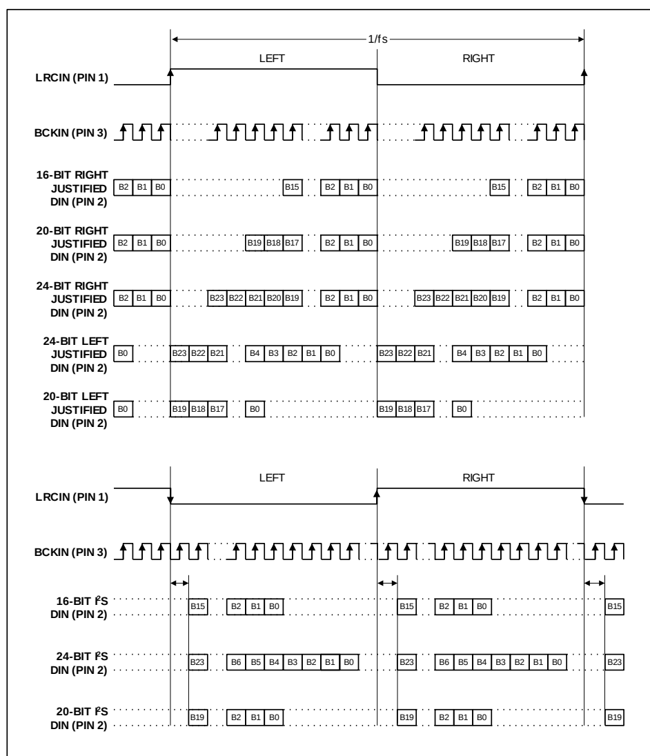
Figure 8 Audio Data Input Format
