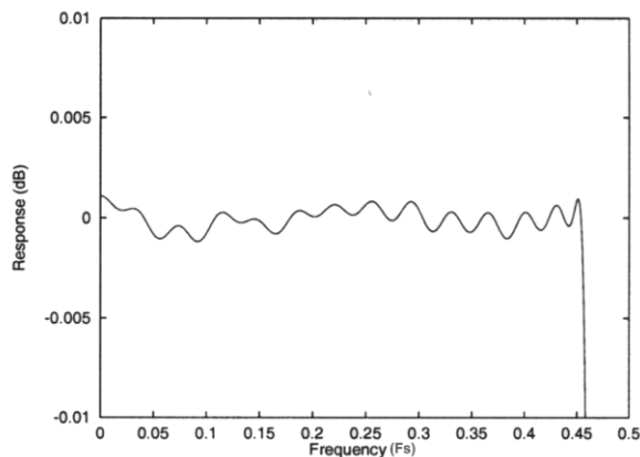
Figure 13 Digital Filter Response (Sharp Roll-off Mode)
