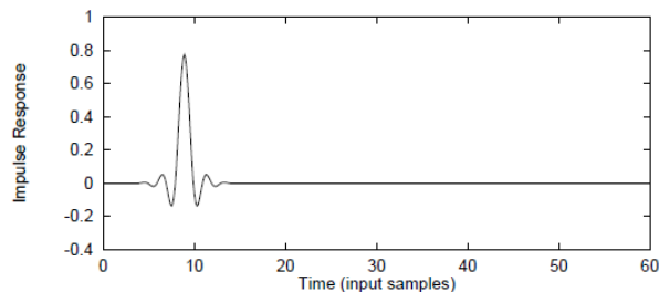
Figure 18 Impulse Response (Slow Roll-off, no De-emphasis)
