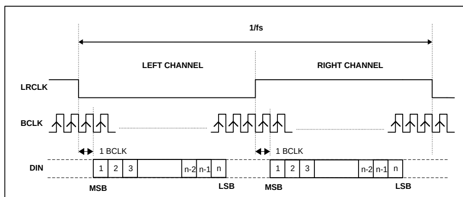
Figure 16 I 2 S Mode Timing Diagram
