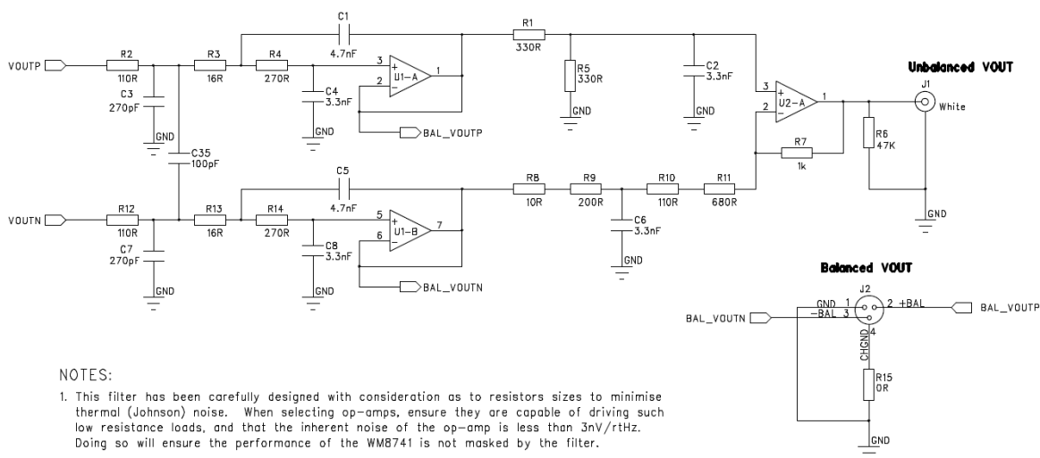
Figure 82 External Components
