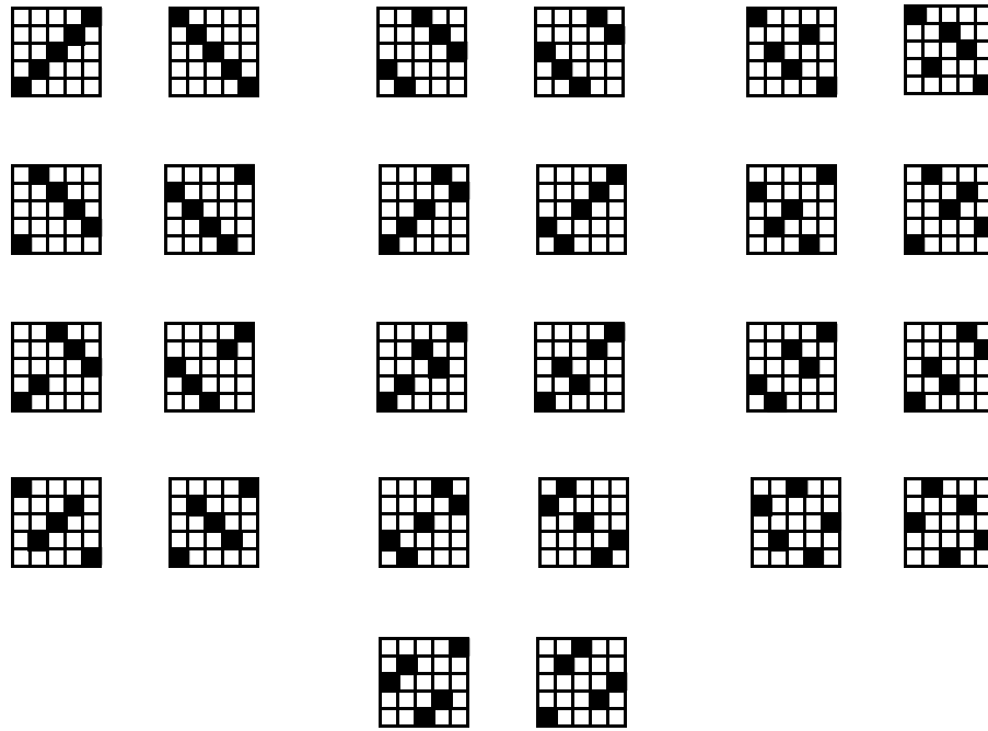
Figure 1. All Possible Involution Patterns for Five Blocks
