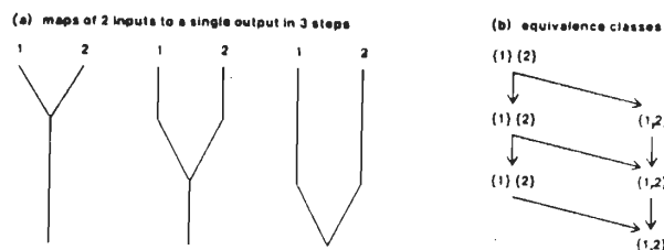
FIG. 2. (a) The three ways of mapping two inputs to a single output in three steps represented as trees. (b) Corresponding equivalence classes. Each of the three paths through the classes corresponds to a specific map.
