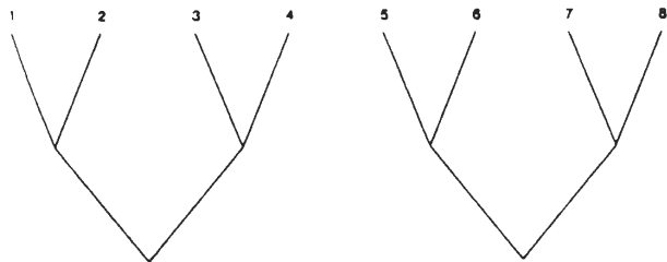
FIG. 5. Example of two balanced binary trees corresponding to a two-step map. Each tree has four inputs and the total number of inputs is n = 2 \times 2^2 = 8 .
