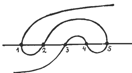
meander 34521
