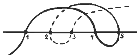
not meander 14523
