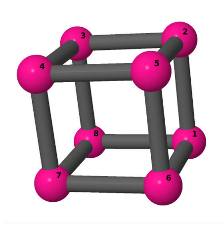
FIGURE 4. Structure of the cubical graph with 8 vertices and 12 edges.
