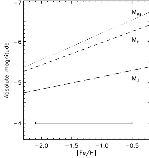
Figure 2. The relationship between the theoretical TRGB magnitude and [\text{Fe}/\text{H}] from Yonsei-Yale isochrones. The long-dashed, short-dashed, and dotted lines are the relations in JHK_S bands. Horizontal bar represents the adopted metallicity range of IC 1613.
