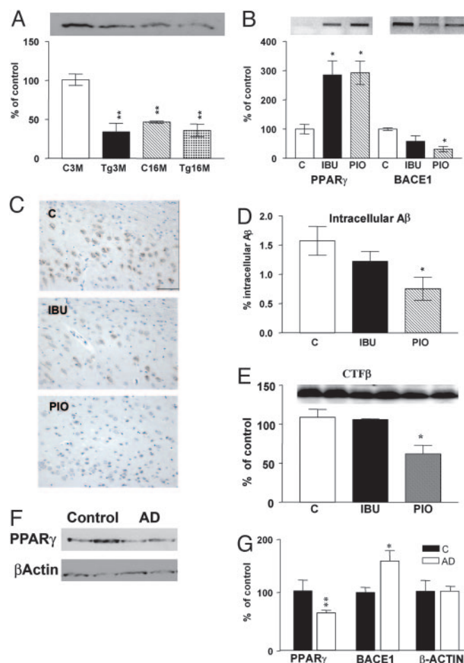
Fig. 4. PPAR \gamma in the brain of APPV717I transgenic mice and in AD patients. (A) Quantification of PPAR \gamma expression in cortex from mouse brain control and APPV717I of 3 and 16 months of age. (B) Quantification of the mRNA levels of PPAR \gamma and BACE1 APPV717I mice treated with ibuprofen (IBU) and pioglitazone (PIO). (C) Immunostaining of intracellular A \beta in subiculum from APPV717I mice treated with IBU and PIO. (D) Quantification of percentage of intracellular A \beta in subiculum from APPV717I mice treated with IBU and PIO. Bar, 100 \mu M. Columns represent mean \pm SEM, n = 4 . (E) Representative Western blot for CTF- \beta fragments in cortex from APPV717I mice treated with IBU and PIO. (F) Representative Western blot for PPAR \gamma expression in brain lysates from two control and two AD patients. As a negative control, \beta -actin expression was analyzed. (G) Quantification of the levels of \beta -actin, PPAR \gamma , and BACE1 in the frontal cortex of 10 controls and 10 AD patients. Asterisks, significant differences between control and AD. *, P \leq 0.05 ; **, P \leq 0.01 . ANOVA followed by a Tukey post hoc test or Student's t test for human brains.
