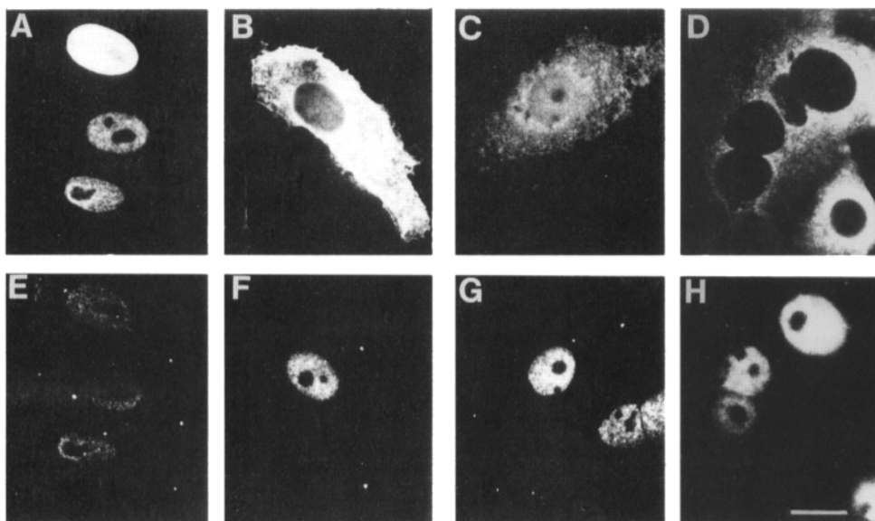
Figure 6. FS T antigen does not interfere with the nuclear import of DIG-U1 snRNAs. Vero cells were microinjected in the nucleus with plasmid DNA encoding wild-type (A and E), cT.3 (B and F), FS (C and G), or cTFS (D and H) T antigen. 6 h later, the same cells were microinjected in the cytoplasm with DIG-U1 snRNA. The cells were incubated for an additional 6 h at 37°C and then prepared for double indirect immunofluorescent staining. A rabbit anti-serum directed against T antigen and a Texas red-conjugated second antibody were used to visualize T antigen (A-D). Mouse antidigoxigenin and an FITC-conjugated second antibody were used to visualize DIG-U1 snRNA (E-H). Bar, 10 \mu m.
