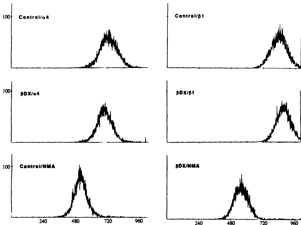
Figure 2. Inhibition of CSPG synthesis by \beta D \times does not affect cell surface expression of \alpha 4 \beta 1 integrin. Cultured melanoma cells were preincubated (or not) with 1 mM \beta D \times for 24 h as described in Materials and Methods. Cultured cells were then released using EDTA and incubated with anti- \alpha 4 integrin mAb (P4C2), anti- \beta 1 integrin mAb (P4C10), or normal mouse ascites (NMA) at final dilutions of 1:100 for 30 min at room temperature. Cells were washed three times, incubated with FITC goat anti-mouse IgG at a final dilution of 1:250 for 30 min at room temperature and then analyzed by flow cytometry.
