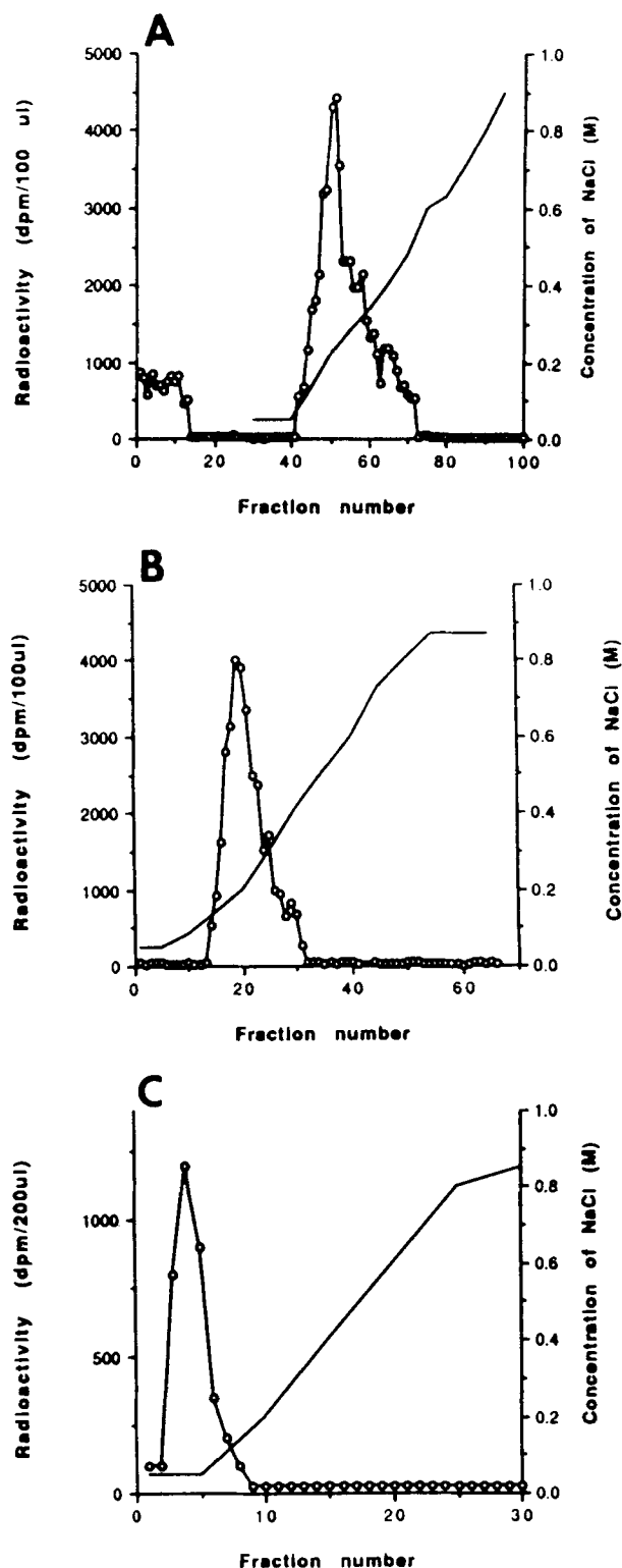
Figure 7. Peptides FN-C/H-I and FN-C/H-II, but not CS1, bind purified melanoma cell CSPG. Affinity columns containing (A) FN-C/H-I/OVA, (B) FN-C/H-II/OVA, or (C) CS1/OVA were evaluated for their ability to bind purified CSPG from melanoma cells. The purified CSPG was applied to these affinity columns in buffer containing 0.05 M NaCl as described in Materials and Methods. The columns were then eluted with a 0.05 to 0.8 M gradient of NaCl (—). The recovery from each affinity column was 95%. Nonspecific binding of the CSPG samples, as judged by their ability to bind to OVA/OVA sham affinity columns, was less than 5% of the total radioactivity applied under these conditions.
