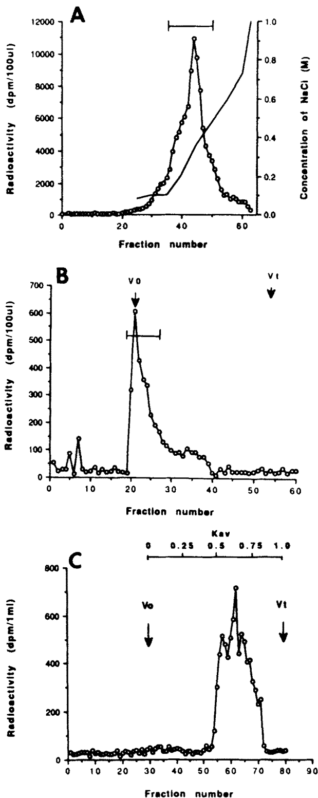
Figure 1. A375 SM human melanoma cells express predominantly CSPG. Cell cultures were metabolically labeled overnight in the presence of 50 \mu Ci/ml of [ ^{35} S]sulfate and the cell layer was subsequently harvested and dialyzed. (A) The dialyzed extract was then applied to a DEAE-Sephacel column and eluted using a linear NaCl gradient from 0.1 to 0.8 M as indicated (—). The radioactive fractions were then pooled (indicated by the bracket), dialyzed, and lyophilized. (B) The pooled fractions were applied to a Sepharose CL-4B column under dissociative conditions. The indi-
