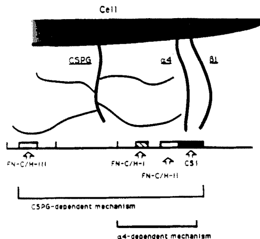
Figure 9. Schematic diagram illustrating a coordinated role for CSPG-dependent and \alpha 4 \beta 1 integrin-dependent cellular recognition sites in mediating melanoma cell adhesion to the 33-kD fragment. Schematically depicted is a human melanoma cell initially recognizing substrata coated with the 33-kD fragment of human plasma FN-A-chains. The three type III repeating homologies (12, 13, and 14) and a portion of the type IIICS insert are depicted, as are the relative locations of the four synthetic peptides used in this study. According to this model, the proximity of the CSPG-dependent and \alpha 4 \beta 1 -integrin-dependent elements, within the context of a larger cellular recognition domain within this fragment, would act to focus cell surface CSPG and \alpha 4 \beta 1 integrin on the ventral surface of the plasma membrane. This clustering of cell surface receptors would act to modulate early cellular events that contribute to melanoma cell adhesion on this fragment. Evidence for this model is summarized in the Discussion.
