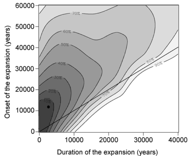
Figure 4. Onset and duration of the demographic expansion. Plot of the joint posterior distribution for the time of onset of the expansion, t_0 , and the length of the expansion, t_0-t_1 . Computations were performed under demographic Model C, in which the population was initially constant, then grew exponentially until t_1 , and then remained constant until the present. Percentages represent the cumulative probabilities under the density curve. The straight line indicates that the duration of expansion cannot be longer than the time elapsed since the onset of expansion.
