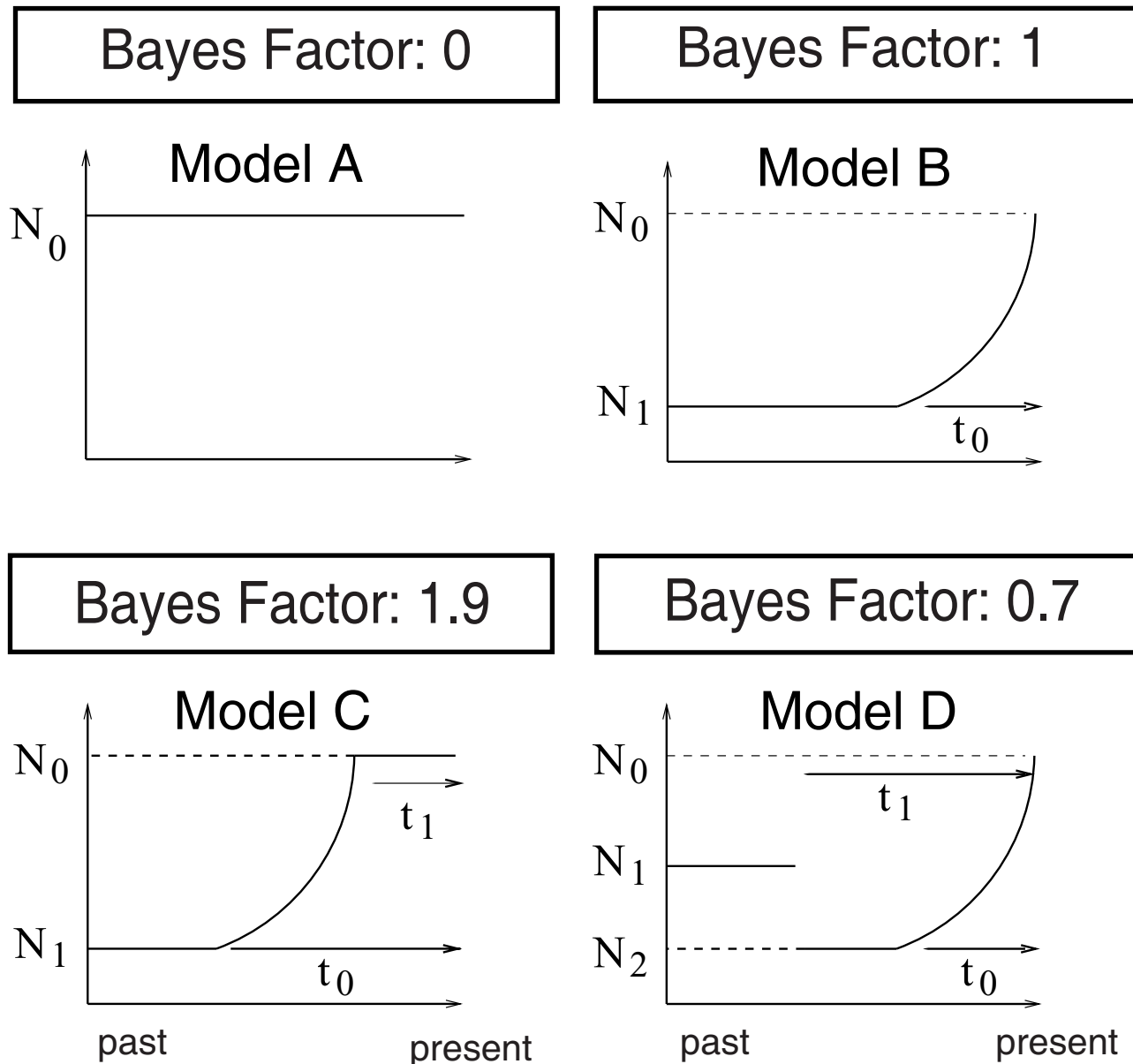
Figure 3. Bayes factors. The 4 demographic scenarios (Models A–D) and their associated Bayes factors. Model A is the model with constant population size, N_0 . Model B is a model with an exponentially growing population size (present size, N_0 , ancestral size, N_1 , time since the onset of expansion, t_0 ). In Model C, the growth is exponential between two periods with constant size (present size, N_0 , ancestral size, N_1 , time since the onset of expansion, t_0 , time since the end of expansion, t_1 ). Model D is similar to Model B, but it includes an ancient bottleneck before expansion. Variants of these 4 models, including variable mutation rates across loci, are considered here. The Bayes factors (top boxes) correspond to the ratio of the weight of evidence of each model to the weight of evidence of Model B. Two window sizes, \delta_{0.01} and \delta_{0.05} , were used when computing the Bayes factors. These window sizes correspond to the 1% and 5% quantiles of the distance between the values of the summary statistics obtained under Model B and the observed values of the summary statistics. The Bayes factors were identical for the 2 window sizes and for values rounded for one decimal place, except for Model C, for which a minor difference was observed (1.8 for \delta_{0.05} instead of 1.9). doi:10.1371/journal.pgen.1000075.g003
