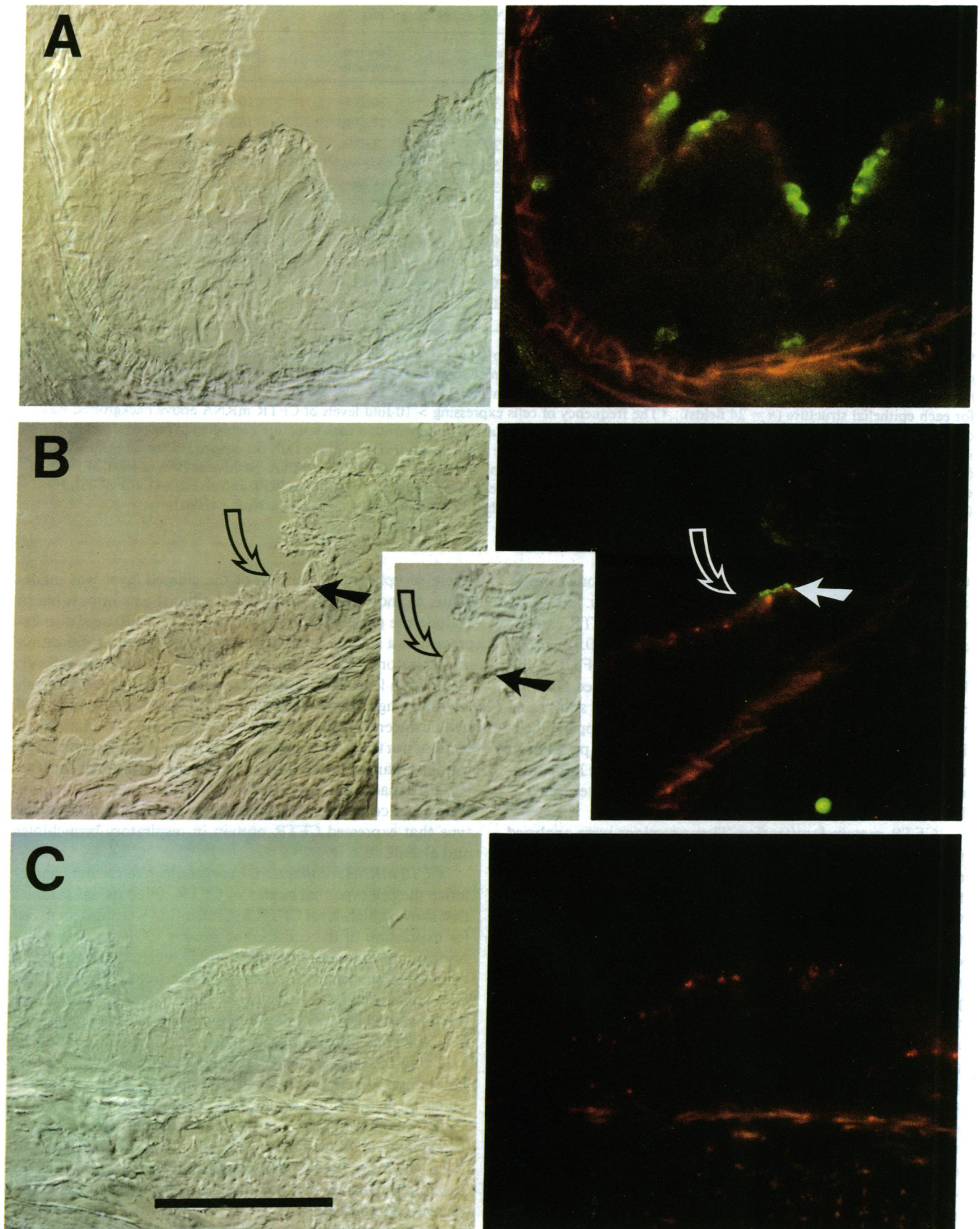
Figure 2. Peptide competition of CFTR protein localization in bronchioles. Immunocytochemical localization of CFTR protein expression in lung sections was analyzed by peptide competition in serial section. (A) Pattern of CFTR expression detected with FITC within a proximal bronchiole in the absence of peptide antigen. Shown are localization of CFTR within serial sections of a terminal bronchioles in the absence of peptide antigen (B) and after preincubation of the \alpha 1468 antibody with peptide antigen (C). The open arrows mark a ciliated cell, while the filled arrows mark a CFTR-expressing nonciliated cell. Each set consists of a Nomarski (left) and immunofluorescent (right) photomicrograph (bar = 53 \mu m).
