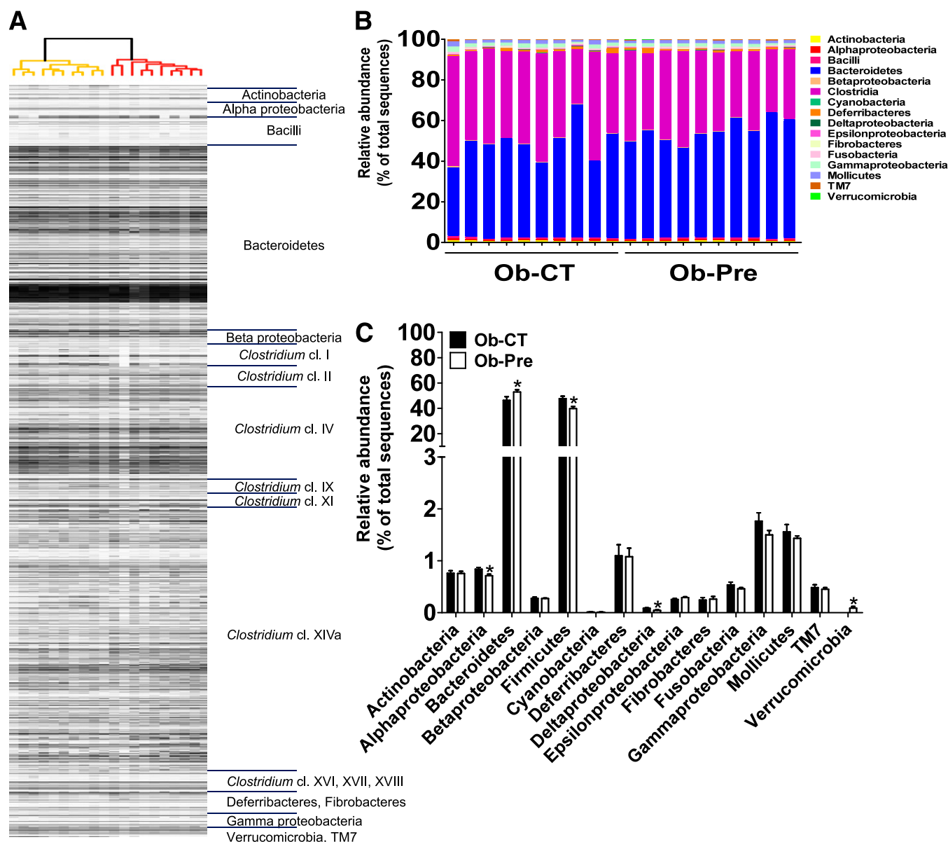
FIG. 2. Phylogenetic microarray analysis of gut bacterial community from the Ob-CT and the Ob-Pre mice. A: Clustering of the MITChip phylogenetic fingerprints of the gut microbiota from the cecal content of the Ob-CT and the Ob-Pre mice ( n = 10 /group). The highest phylogenetic level of specificity of probes (level 1) is depicted on the right. B: Percentage of each community contributed by the indicated taxa. C: Relative abundance of different taxa expressed as the percentage of total sequence reads. Mean \pm SEM. n = 10 mice/group. * P < 0.05 , determined by a two-tailed Student t test.
