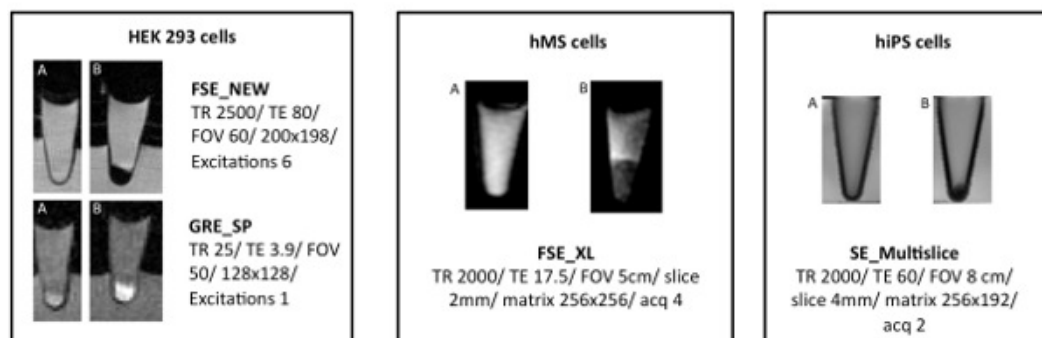
Figure 2. MR images of sagittal cross sections through eppendorf tubes with cells in a cell pellet. A) Unlabeled controls. B) Labeled cells demonstrating a significant T2 or negative contrast agent effect on T2-weighted FSE or SE_Multislice imaging and a T1 or positive contrast agent effect on the T1-weighted GRE sequence.
