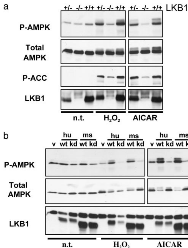
Fig. 2. LKB1-deficient MEFs are defective in AMPK activation. (a) Littermate MEFs of the indicated LKB1 genotypes were left untreated (n.t.) or were treated with 0.1 mM H_2O_2 for 20 min or 2 mM AICAR for 2 h. Total cell extracts were immunoblotted for phospho-Thr-172 AMPK (P-AMPK) or phospho-Ser-79 ACC (P-ACC), as well as for total AMPK and LKB1. (b) An immortalized LKB1-deficient MEF cell line was reconstituted with human (hu) or mouse (ms) WT (wt) or kinase-dead (kd) LKB1-expressing retroviruses. v, Vector control cells; hu wt, human FLAG-tagged WT LKB1-expressing cells; hu kd, human FLAG-tagged kinase-dead LKB1-expressing cells; ms wt, untagged mouse WT LKB1-expressing cells; ms kd, untagged mouse kinase-dead LKB1-expressing cells. Cells were treated as in a. The asterisk indicates a background band that serves as a loading control.
