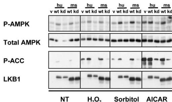
Fig. 3. LKB1 regulates activation of AMPK in response to the AMP analogue AICAR as well as to oxidative or osmotic stress in HT1080 cells. HT1080 cells stably expressing WT or kinase-dead (kd) LKB1 as in Fig. 2 were treated with 0.1 mM H_2O_2 for 20 min, 0.6 M sorbitol for 30 min, or 2 mM AICAR for 2 h. Total cell extracts were analyzed as in Fig. 2. v, Vector control cells; hu, human; ms, mouse; P-AMPK, phospho-Thr-172 AMPK; P-ACC, phospho-Ser-79 ACC.
