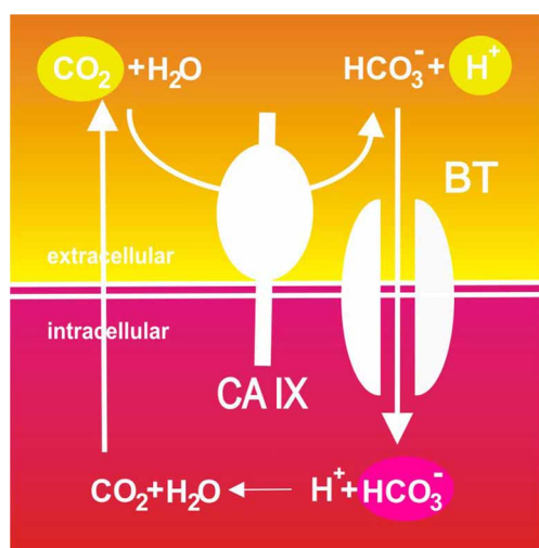
FIGURE 2 | Schematic illustration of the catalytic role of CA IX in pH regulation in tumor cells. Pericellular \text{CO}_2 is hydrated to bicarbonate ions and protons in a reaction efficiently catalyzed by the hypoxia-induced CA IX. Protons remain on the outer side of the plasma membrane and contribute to extracellular acidification. On the other hand, CA IX-facilitated production of bicarbonate ions is spatially and functionally coupled to their inward transport across the plasma membrane through bicarbonate transporters (BT) where these ions consume cytoplasmic protons and neutralize intracellular pH. This results in production of \text{CO}_2 that leaves the cell by diffusion and may enter a new round of hydration.
