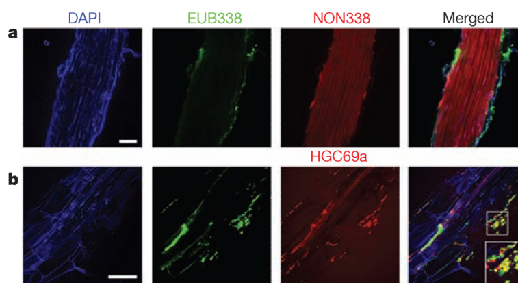
Figure 4. CARD-FISH confirmation of Actinobacteria on roots
