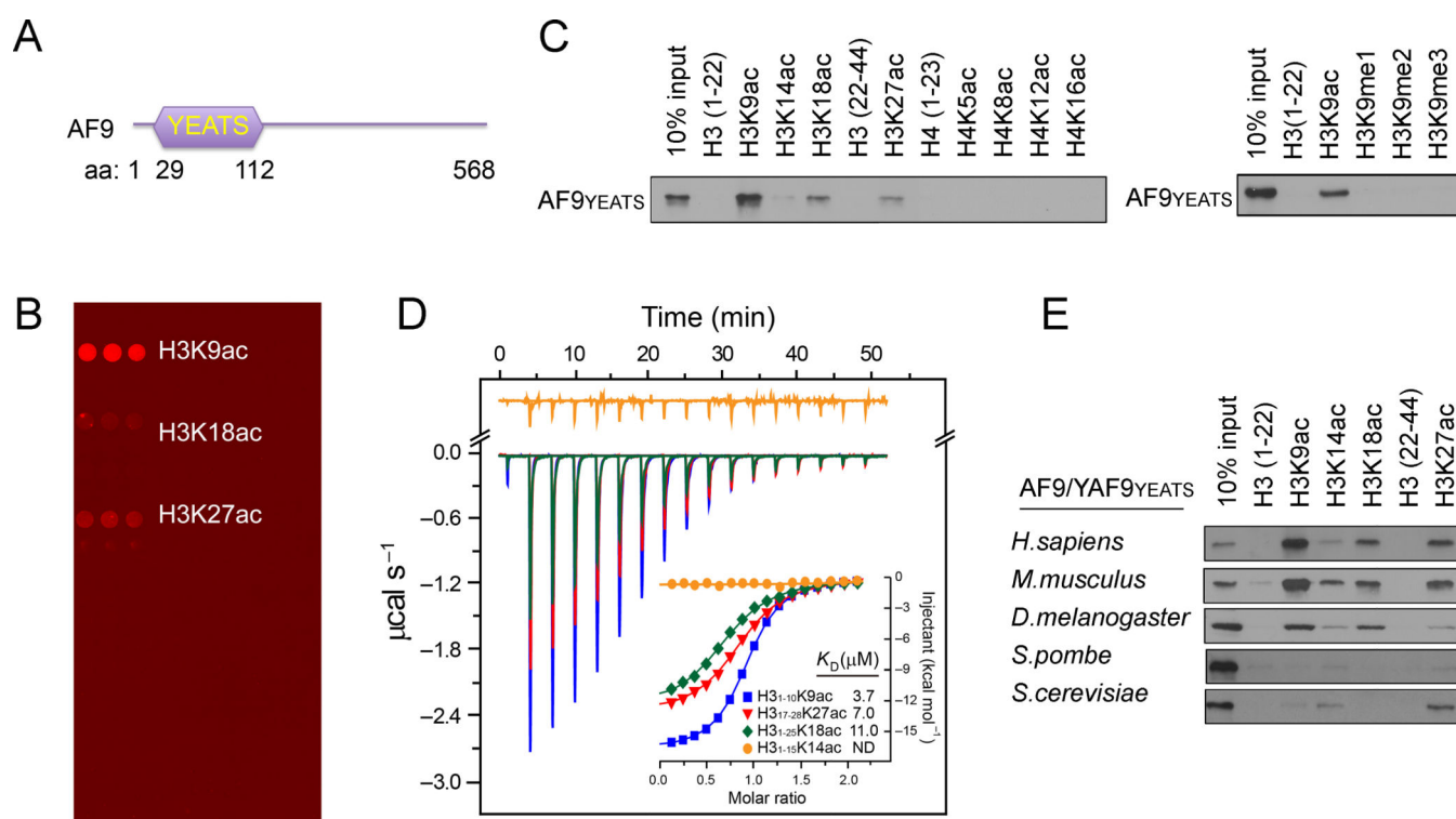
Figure 1. The AF9 YEATS Domain Is a Novel Histone Acetylation-Recognizing Module
