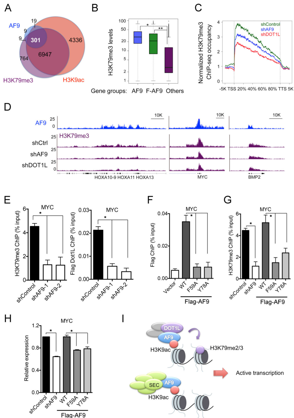
Figure 7. AF9 Is Required for DOT1L-Dependent H3K79me3 Deposition and Gene Activation (A) Venn diagram showing the overlap of AF9-, H3K9ac- and H3K79me3-occupied genes. P < 3.0 \times 10^{-82} (3-way Fisher's exact test).
