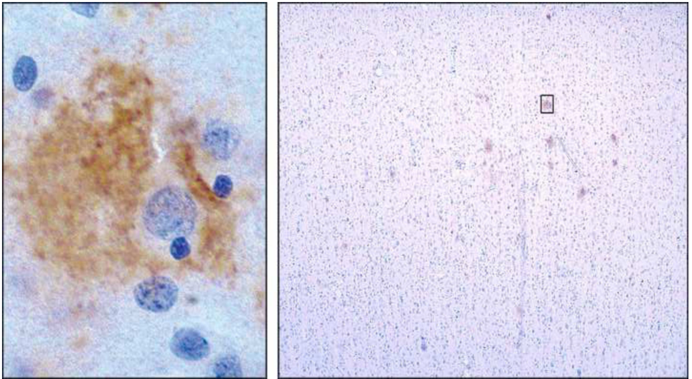
Figure 1. Dendritic oligomer pathology occurs early in disease progression
