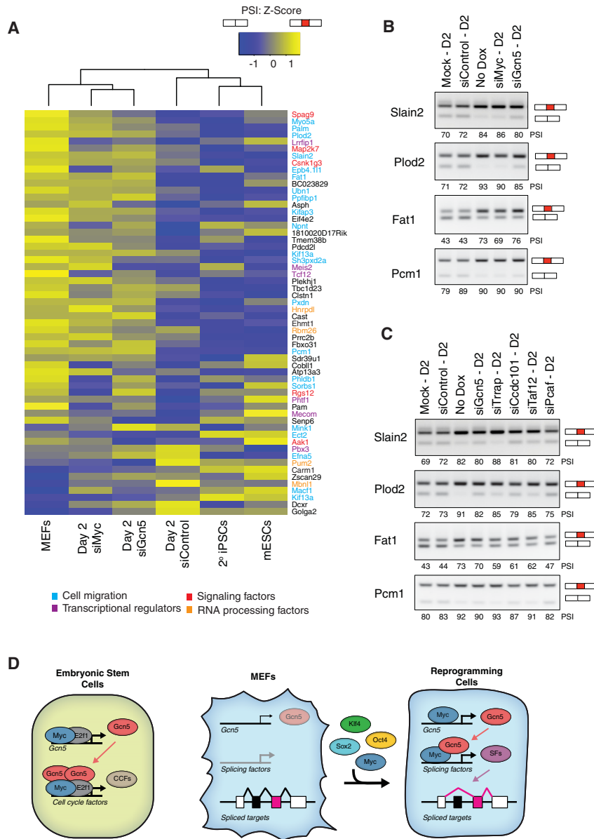
Figure 7. Gcn5 and Myc mediate an AS program during early reprogramming. (A) Heat map of Z-scores from PSI values in MEFs and D2 reprogramming cells transfected with siRNAs targeting Myc and Gcn5 and a nontargeting control. The average of two samples sets is plotted for 59 splicing events. The scale indicates high (yellow) to low (blue) PSI values. The biological functions of select genes are highlighted by color. (B,C) RT-PCR assays monitoring mRNA splicing levels of Slain2 , Plod2 , Fat1 , and Pcm1 in MEFs and D2 reprogramming cells after knockdown of Myc or Gcn5 (B) or knockdown of Gcn5, Trrap, Ccdc101, Taf12, or Pcaf (C). Semi-quantitative PSI values are displayed. The presence of the red exon denotes exon inclusion. Representative images from three independent experiments are shown. (D) Gcn5 and Myc cooperate to initiate a sequence of events centered on RNA splicing in reprogramming cells. (Left) In mESCs, Myc and E2f1 stimulate a feed-forward circuit by enhancing Gcn5 levels so that Gcn5 may occupy cell cycle factor (CCF)-related genes with Myc and E2f1. (Middle and right) At the onset of reprogramming, Myc interacts with the TSS of Gcn5 to stimulate Gcn5 expression and facilitate a positive feed-forward loop. Myc associates with Gcn5 in reprogramming cells to up-regulate the expression levels of splicing factors (SFs). The splicing factors mediate AS, primarily exon exclusion, to advance somatic cell reprogramming.
