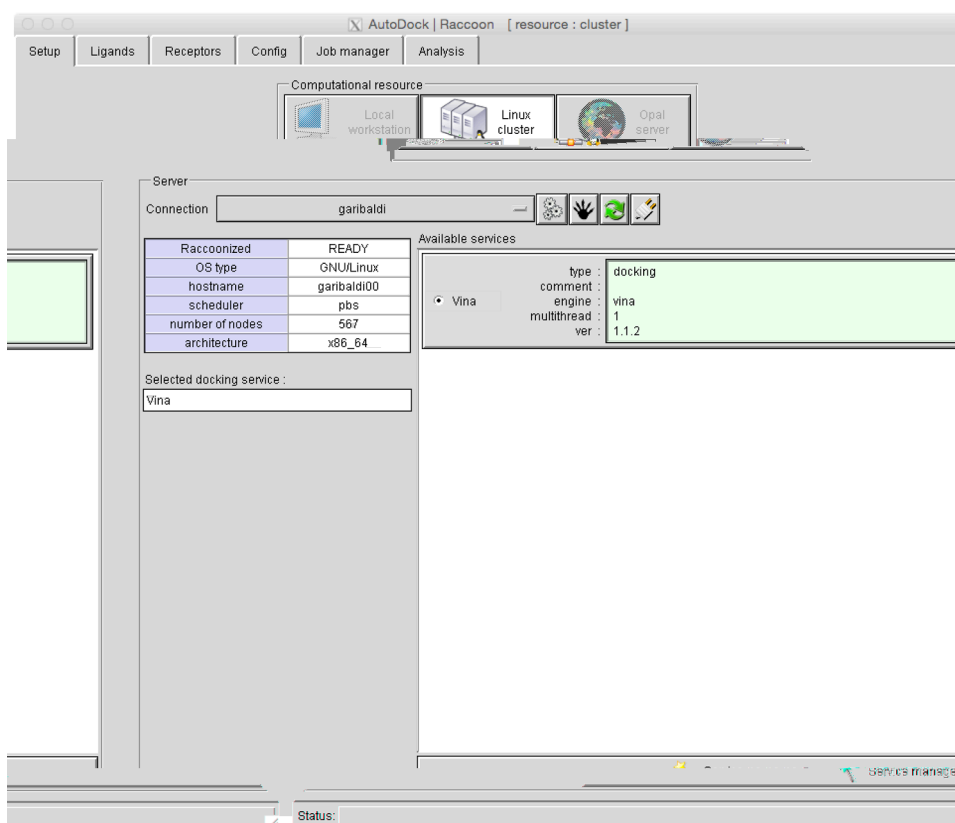
Figure 3. Raccoon2
