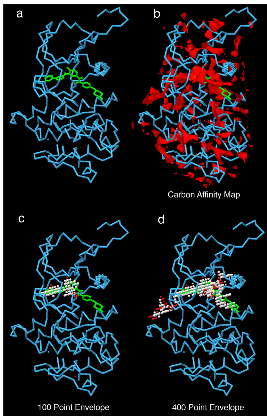
Figure 5. AutoLigand Results
