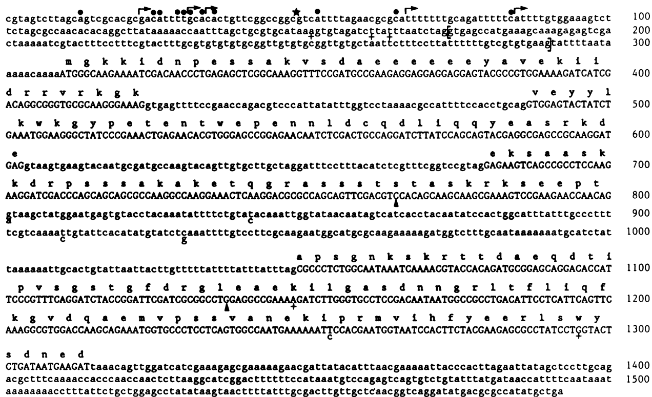
FIG. 4. Genomic sequence of the HP-1 locus. The predicted protein-coding DNA sequence is shown by uppercase letters. Corrections of previously published sequence information (10) are indicated by symbols below the DNA sequence ( \Delta , nucleotide change; +, nucleotide insertion). A star indicates the position at which genomic HP-1 sequence diverges from the upstream sequence of a previously described cDNA. Lowercase letters below the sequence indicate nucleotides found to differ in the Su(var)205 allele. Arrows indicate the first nucleotide of cDNAs recovered from various cDNA libraries; from right to left, the start sites correspond to (i) clones 213 and 321, (ii) clones 343 and 351, (iii) clone 431, (iv) clones pTH1 and pTH5, and (v) clone 243 (see Fig. 5B). Dots above the sequence indicate putative transcription start sites predicted from primer extension analysis using poly(A) + RNA from adult flies. The sequence of the intron within the 5' untranslated region is indicated by brackets. Note the terminal AAG sequence found at the 3' end of this intron.
