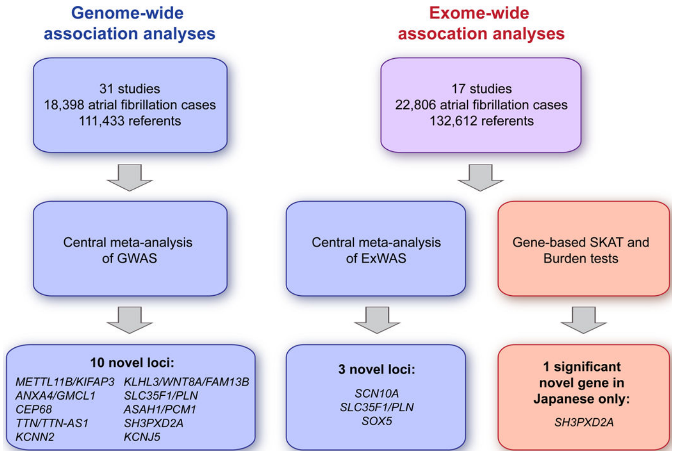
Figure 1. Study flow-chart
