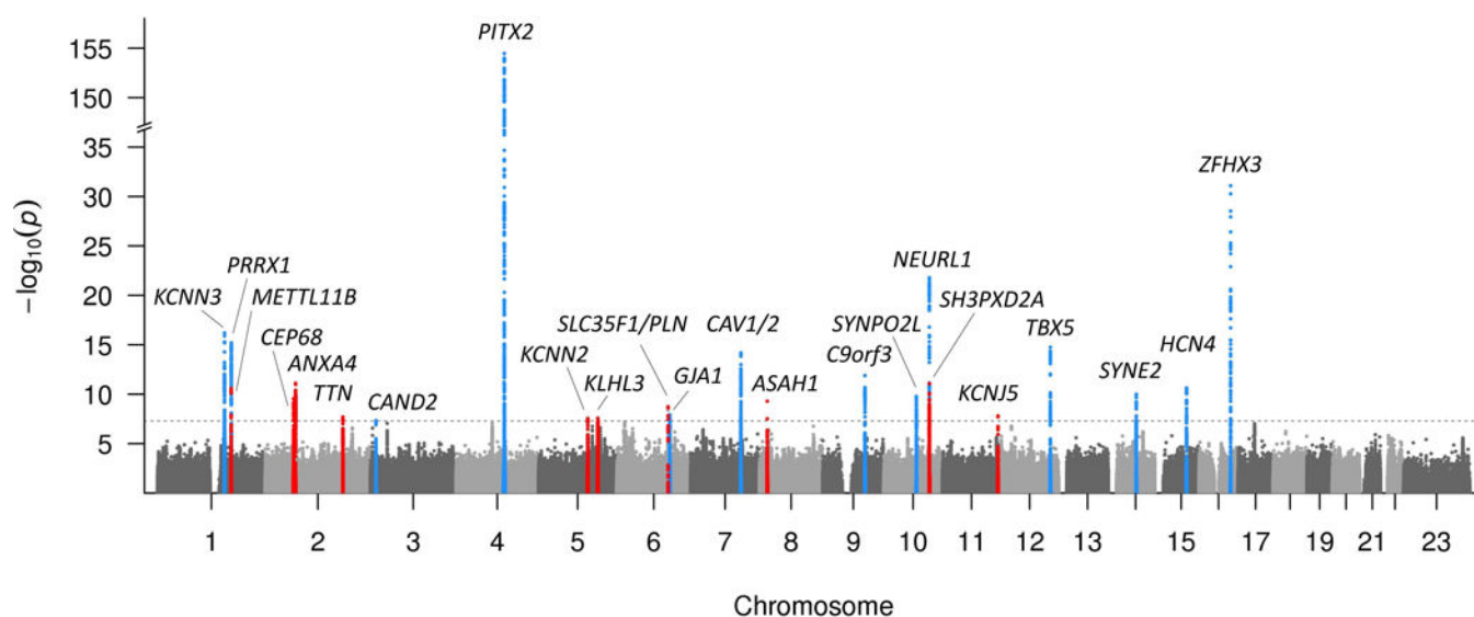
Figure 2. Manhattan plot of the combined ancestry GWAS meta-analyses
