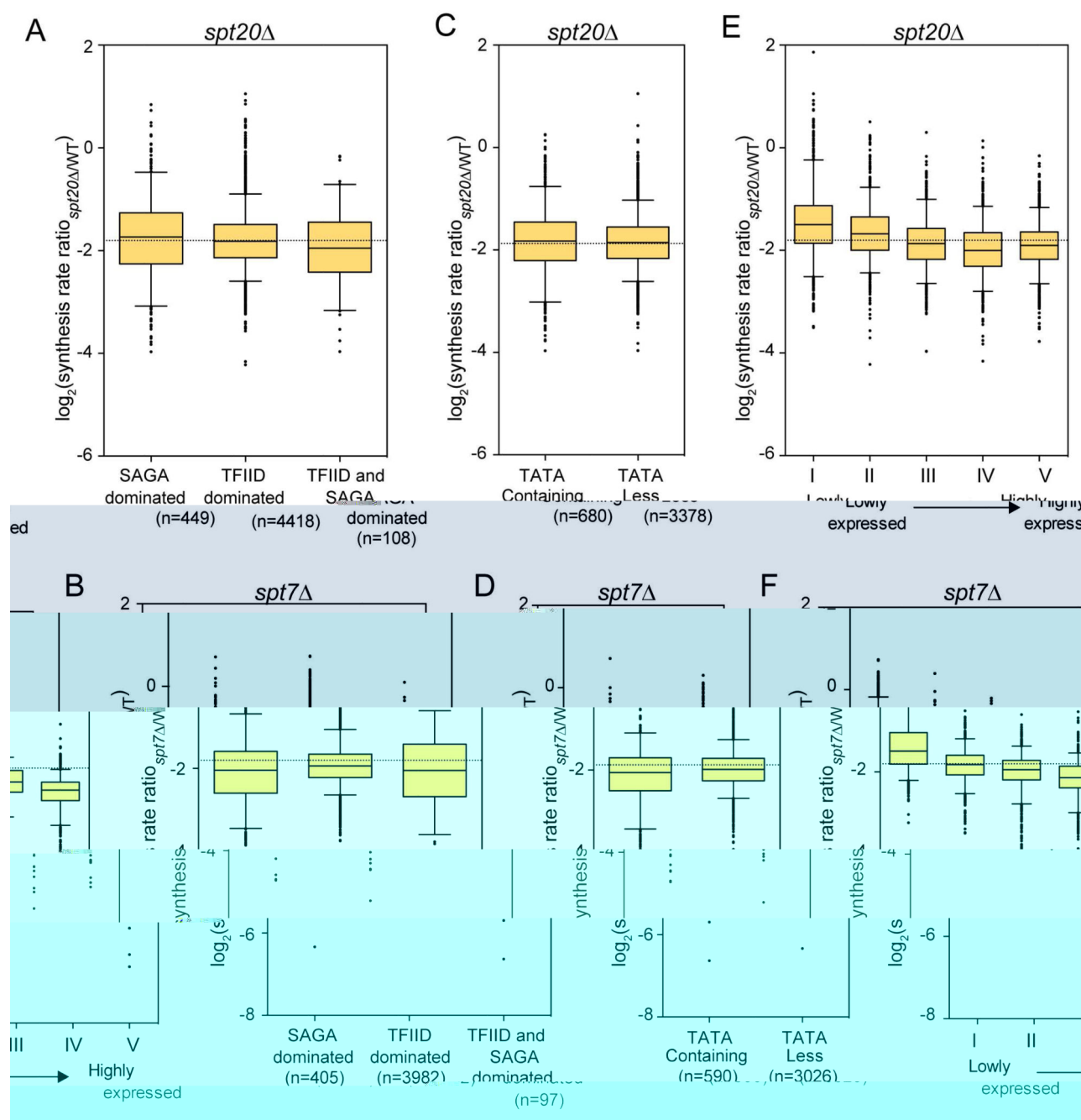
Figure 4. Changes in mRNA synthesis rates for different classes of genes in spt20Δ and spt7Δ . Box plots showing the distribution of changes in mRNA synthesis rates between spt20Δ (A,C,E) or spt7Δ (B,D,F) and wild-type strains. Very similar changes were seen whether genes were described as SAGA- or TFIID-dominated (A,B) or whether their promoter were TATA-containing or TATA-less (C,D). Genes were divided in quintiles according to their expression levels in wild-type cells and the changes in synthesis rates were plotted for each quintile (E,F). Boxes contain genes between the 25 th and the 75 th centiles, the line indicates to the median and the whiskers correspond to 5 th and 95 th centiles.
