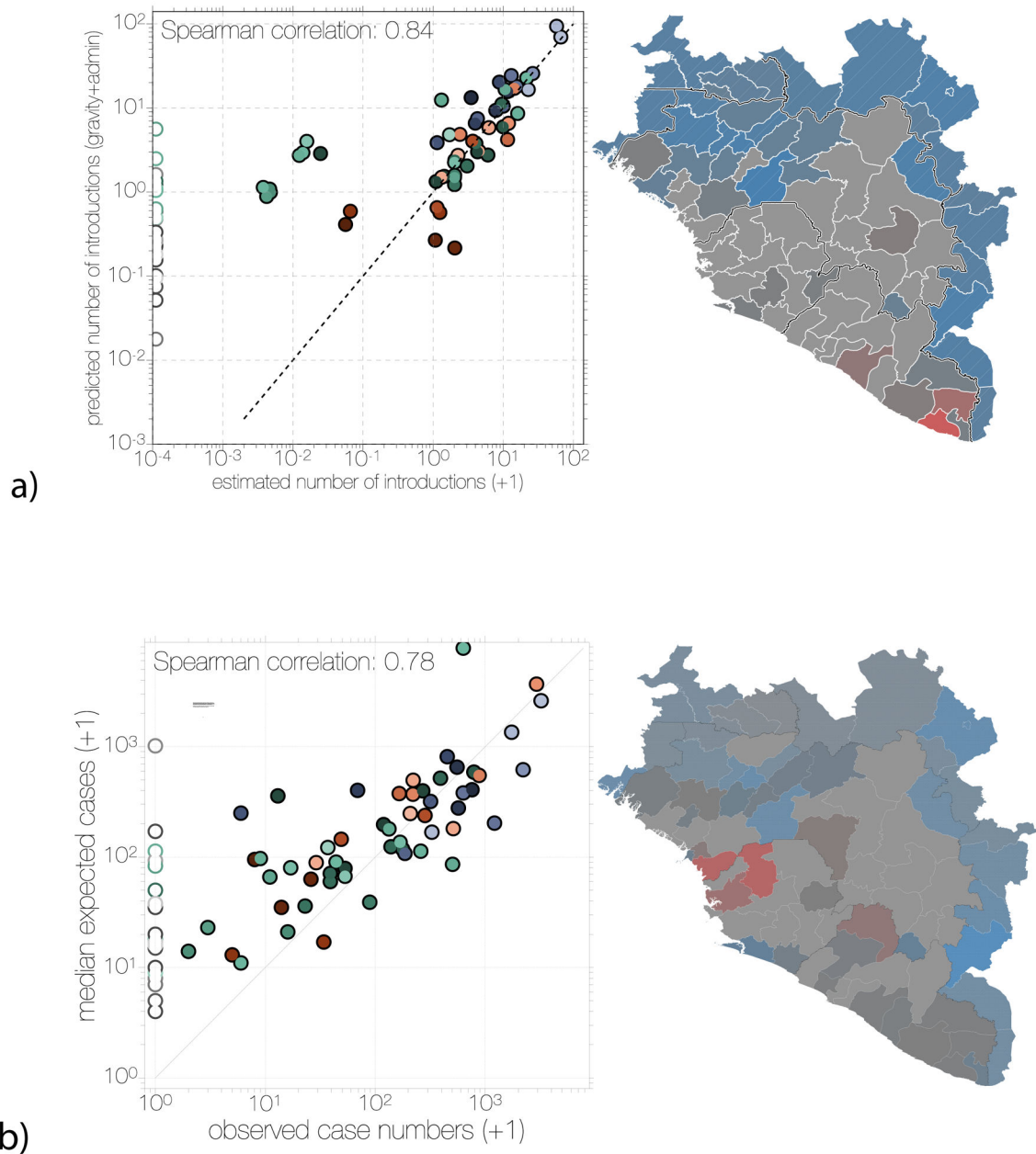
Figure 13. Relationship of cluster size, introductions and persistence to population size
