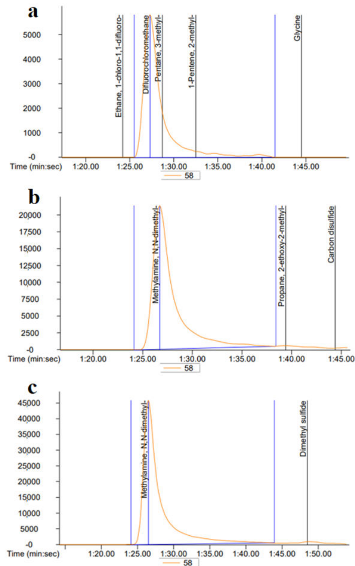
Figure 6. The trimethyl N-oxide (TMAO) was identified and quantified by GC/MS analysis. The representative chromatograms of (a) standard TMAO, (b) raw HDPS, and (c) hot smoked HDPS. The TMAO was identified and quantified by the reference TMAO injecting into the GC/MS. The TMAO spikes in the chromatograms appeared at 1 min 25 s of retention time among different treatment groups.
