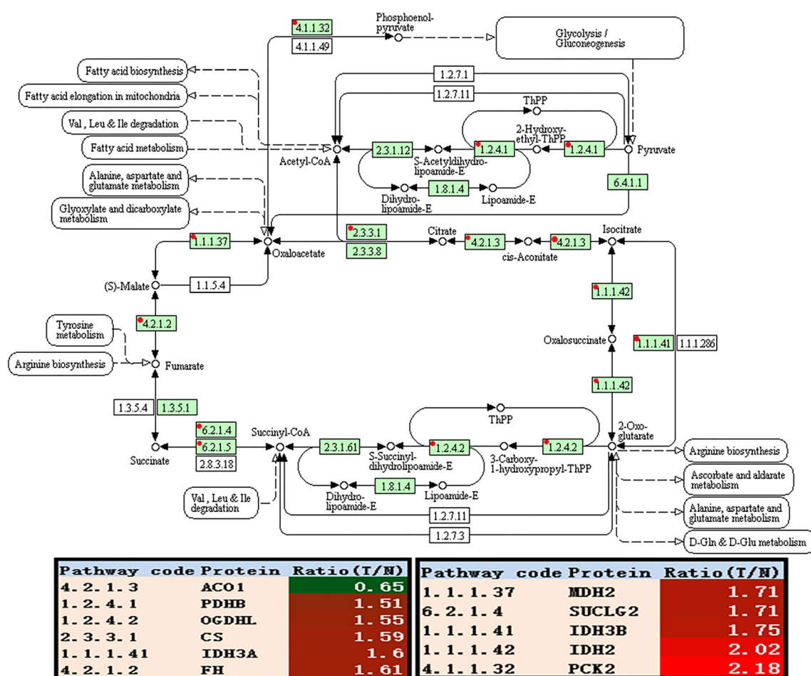
Fig. 3 Krebs' cycle altered in ovarian cancer. Green rectangle without red mark means species-specific enzymes. White rectangle means reference pathway. The solid line means molecular interaction. The dot line means indirect effect. The circle means mostly chemical complex. ACO1, cytoplasmic aconitate hydratase; PDHB, pyruvate dehydrogenase E1 subunit beta; IDH2, isocitrate dehydrogenase (NADP(+)) 2; CS, citrate
