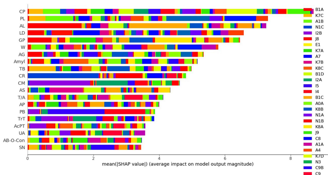
Figure 3. The mean SHAP method result between parameters and disease classifications in XGBoost.
