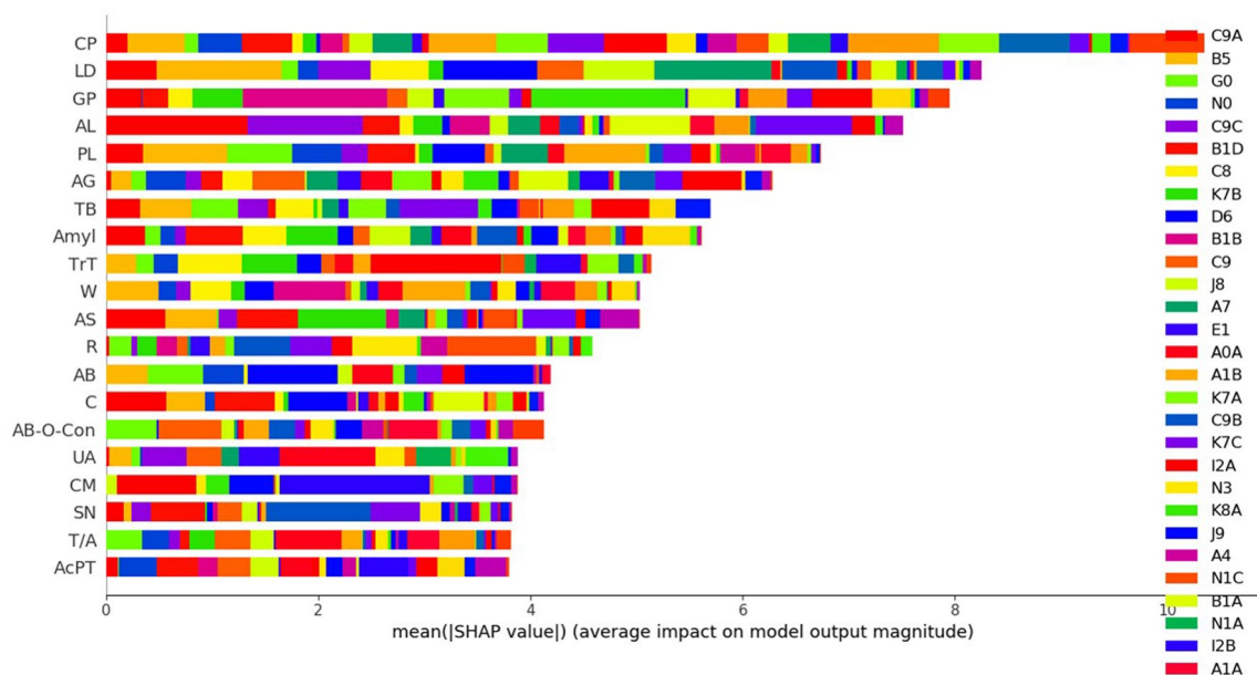
Figure 2. The mean SHAP method result between parameters and disease classifications in LightGBM.
