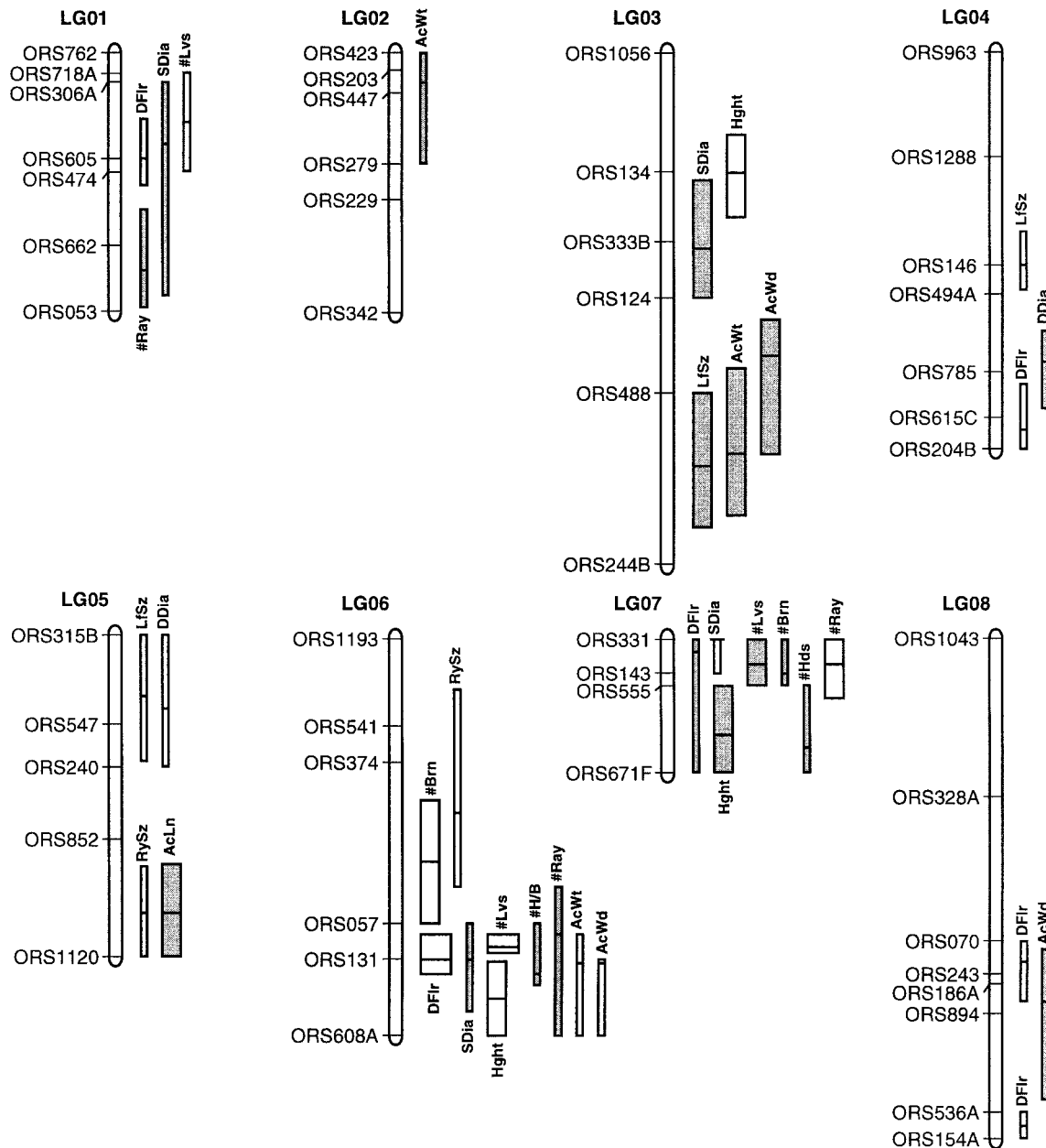
FIGURE 1.—Linkage map derived from the cultivated (cmsHA89) \times wild ( H. annuus var. annuus ) sunflower F_3 mapping population. Marker names are listed to the left of each linkage group, and boxes to the right of each linkage group indicate QTL positions/magnitudes. A horizontal bar marks the most likely position of each QTL within the 1-LOD support limits, and QTL with effects in the expected direction are shaded. Marker names ending in a letter refer to dominant loci, whereas all others are codominant.
