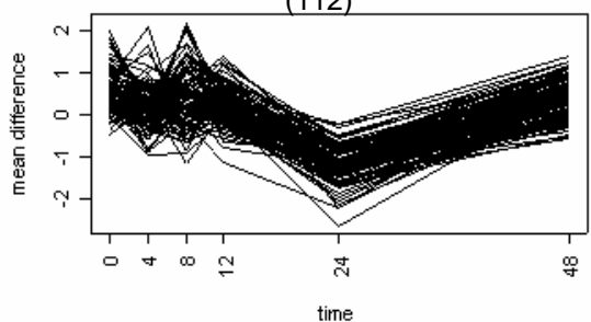
Cluster 8 (112)
