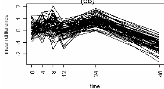
Cluster 11 (68)
