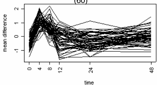
Cluster 10 (60)
