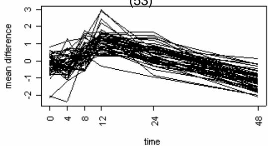
Cluster 12 (53)
