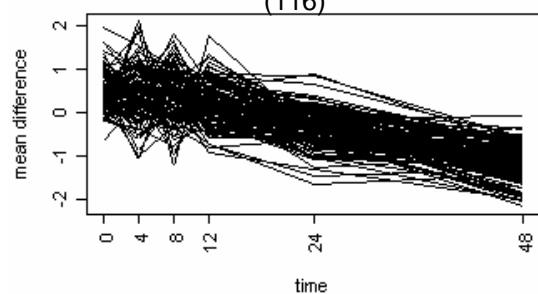
Cluster 9 (116)
