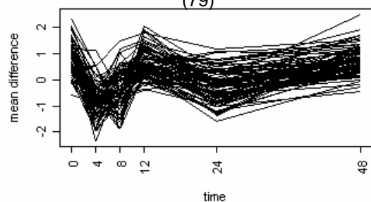
Cluster 7 (79)
