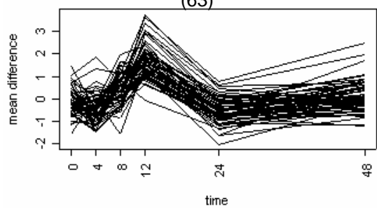
Cluster 25 (63)
