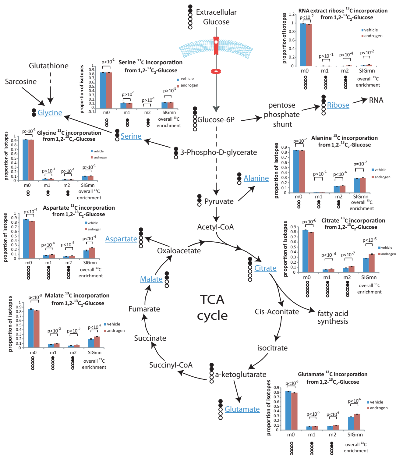
Supplementary Figure 6 Effects of androgen signalling on carbon utilization from glucose in macromolecule biosynthesis. (a) Summary of ^{13}\text{C} incorporation, as assessed by GC/MS analysis of methanol/chloroform extracted LNCaP cell lysates following 48h treatment and 24h incubation of cells with 1,2\text{-}^{13}\text{C}_2 -glucose. Schematic shows simplified glycolysis and TCA pathways, indicating the metabolites which are converted to amino acids for protein synthesis, lipids for fatty acid synthesis and also to ribose for nucleotide synthesis. Black circles depict the carbon atoms of each measured metabolite, filled circles denote ^{13}\text{C} and open circles denote ^{12}\text{C} . The predicted ^{13}\text{C} incorporation based on glucose metabolism directly through glycolysis and the TCA cycle (NB, other routes such as the pentose phosphate pathway would result in other ^{13}\text{C} incorporation rates). Data are presented as mean of technical and biological triplicates ( n=9 ), error bars indicate S.E.M.
