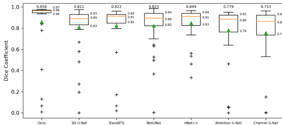
Fig. 1 Comparison of the segmentation performance of different models for all test samples. The numbers at the top represent the mean values of each method (so is the green triangle). The upper, lower quartile, and median values are indicated on the right side of each box plot
