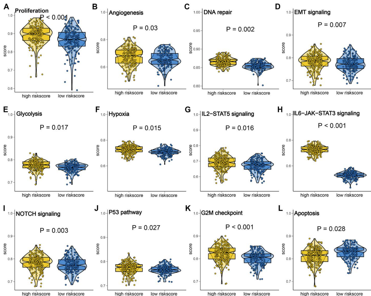
Figure 3. Gene set enrichment analysis of PI3K/Akt pathway related signature (PRS). The gene score of hallmark gene sets correlated with proliferation (A), angiogenesis score (B), DNA repair score (C), EMT signaling score (D), Glycolysis score (E), Hypoxia score (F), IL2-STAT5 signaling score (G), IL6-JAK-STAT3 signaling score (H), NOTCH signaling score (I), P53 pathway score (J), G2M checkpoint score (K) and apoptosis (L) in low and high risk score.
