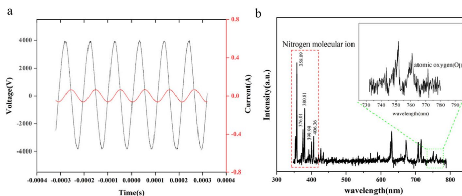
Fig. 1 a Current and voltage waveform of CAP. b Emission spectrum of CAP
