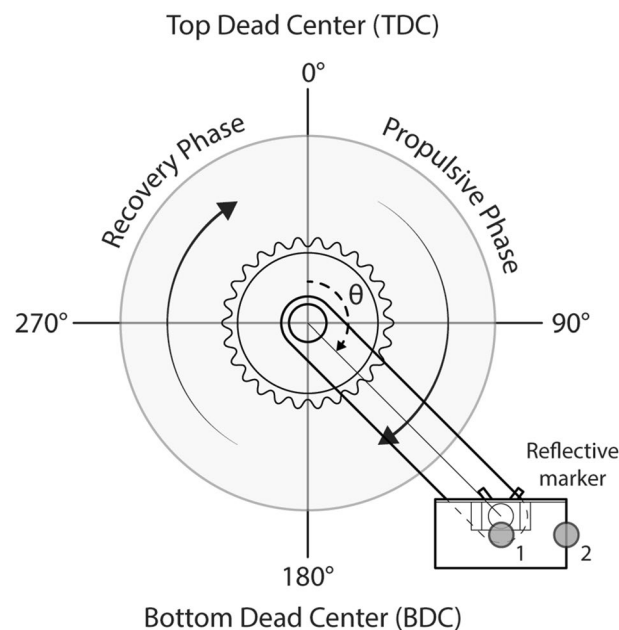
Fig. 6 Schematic illustration of the right pedal. The propulsive phase is from 0° to 180°, and the recovery phase is from 180° to 360°. The gray spheres indicate the location of the reflective marker 1 and marker 2
