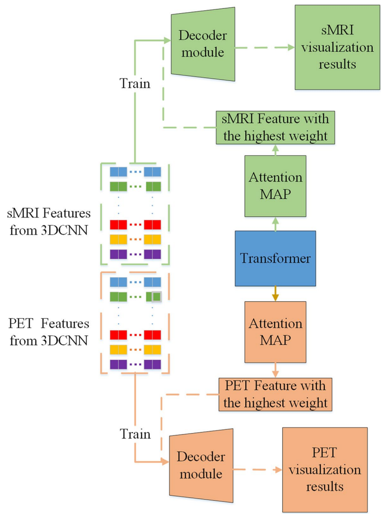
Fig. 8 Visualization framework
