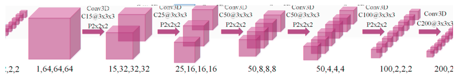
Fig. 4 The architecture of deep 3D CNNs denoted with the sizes of each layer's input, convolution, max pooling, and output layers and the numbers and sizes of generated feature maps. C is a convolutional layer, the P is max pooling layer, @ is the number of filters such as 15@3×3×3 is 15 filters whose size are 3×3×3 and P 2×2×2 is pooling layers, with a size of 2×2×2. The number below each layer represents the shape of the feature
