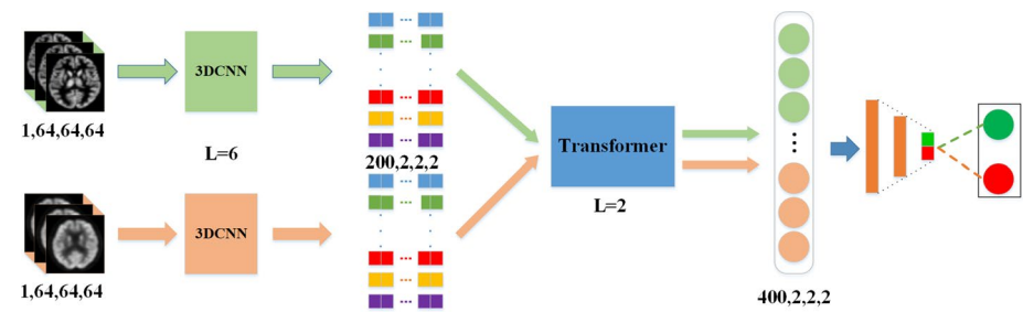
Fig. 7 The framework of network model
