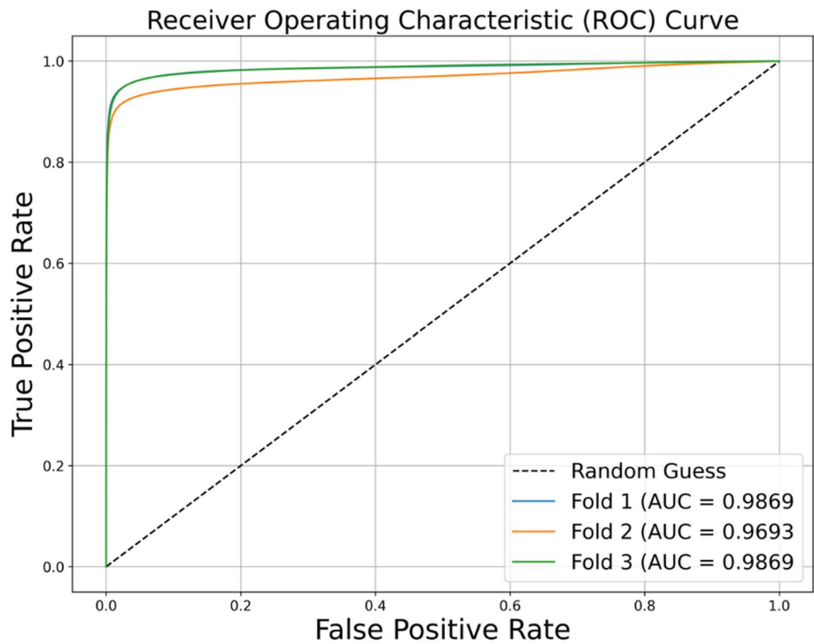
Fig. 2 ROC curve analysis. ROC curve showcases the performance of the setup, indicating its ability to achieve high true-positive rates whilst maintaining low false-positive rates. The average AUC across the threefold is 0.98, with a standard deviation of 0.0082
