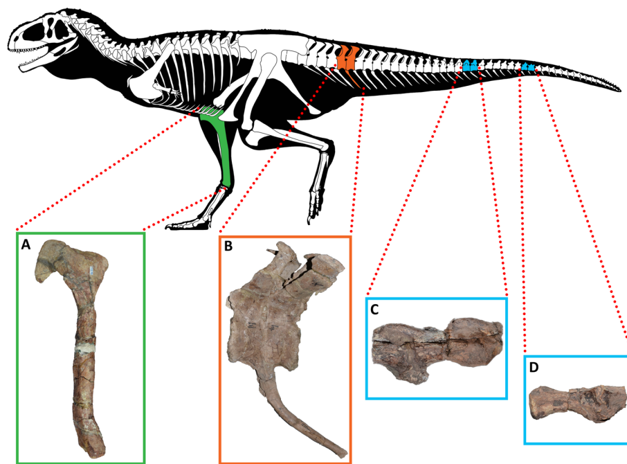
Fig. 1 Elements of Patagonian abelisaurids affected by pathology. A , right tibia of Quilmesaurus curriei MPCA-PV-100 in medial view; B , 5th and 6th caudal vertebrae and 5th haemal arch of Aucasaurus garridoi MCF-PVPH-236, in left lateral view; C and D , middle and posterior caudal vertebrae of Elemgasem nubilus MCF-PVPH-380, in left lateral view. Artwork (silhouette and skeleton) by Alessio Ciaffi
