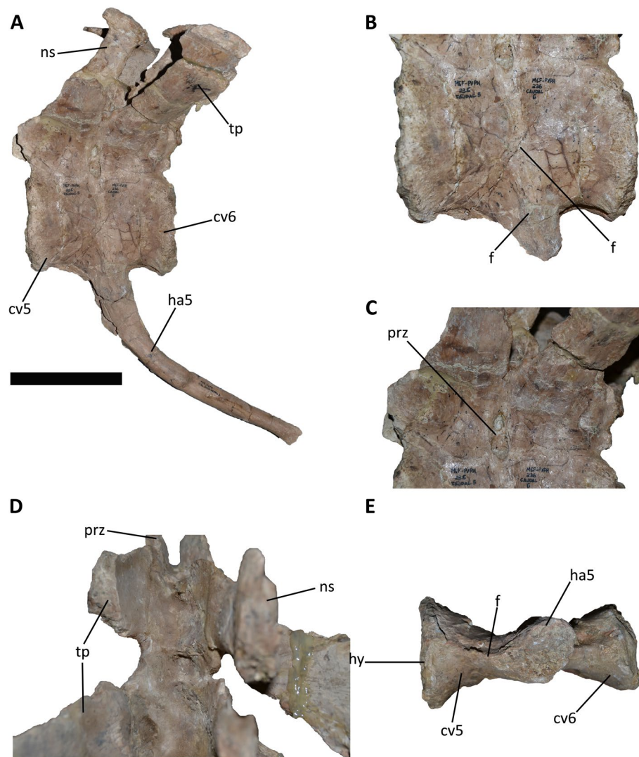
Fig. 2 Fifth and sixth caudal vertebra and fifth haemal arch of Aucasaurus garridoi MCF-PVPH-236. A , the three caudal elements in lateral view; B , detail of fused centra and the haemal arch in lateral view; C , detail of the partial fusion of the neural arches in lateral view; D , detail of the partial fusion of the neural arches in dorsal view; E , detail of the fusion among the three elements in ventral view. Abbreviations: cv5, fifth caudal vertebra; cv6, sixth caudal vertebra; f, fusion of articular surfaces; ha5, fifth haemal arch; hs, contact surface for the haemal arch; ns, neural spine; prz, prezygapophysis; tp transverse process. Scale bar only for the image A: 10 cm
