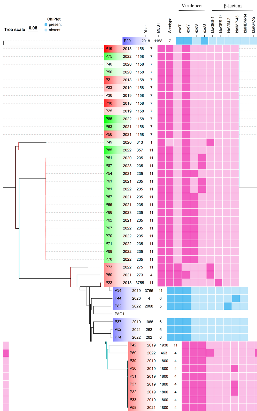
Fig. 2 Molecular characteristics of 47 XDR-hvPA strains. PAO1 (GenBank accession: NC_002516.2) was used as the reference strain
