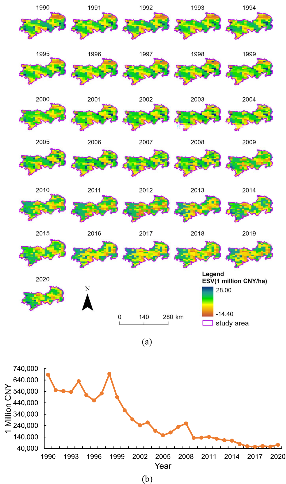
Fig. 3 ESV in the study area, 1990–2020. a Temporal and spatial distribution pattern of ESVd per hectare (b) Changes in total ESVd values in the study area
