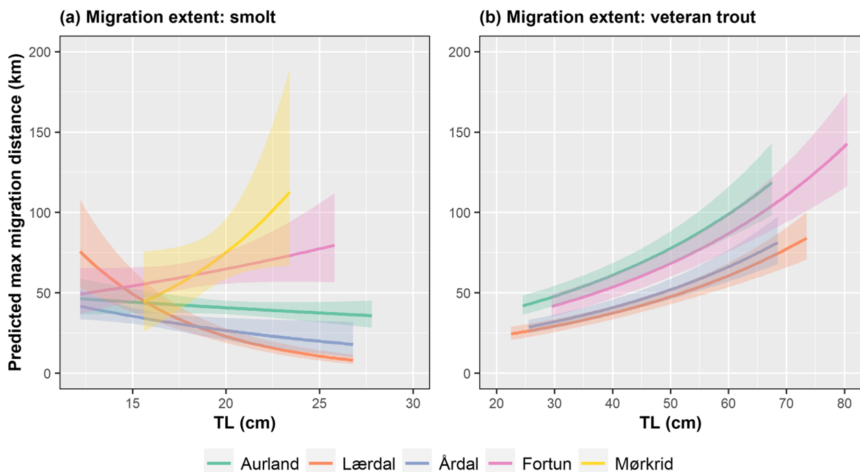
Fig. 4 The effect of natal river and fish length (TL) on predicted maximum seaward migration distance (distance from river mouth) of Sognefjord brown trout smolts ( migration\ distance \sim river*TL ) (a) and veteran migrants ( migration\ distance \sim river + TL ) (b). Note: Models were selected according to AICc; candidate models are listed in Table S2. Model coefficients are stated in Table S3
