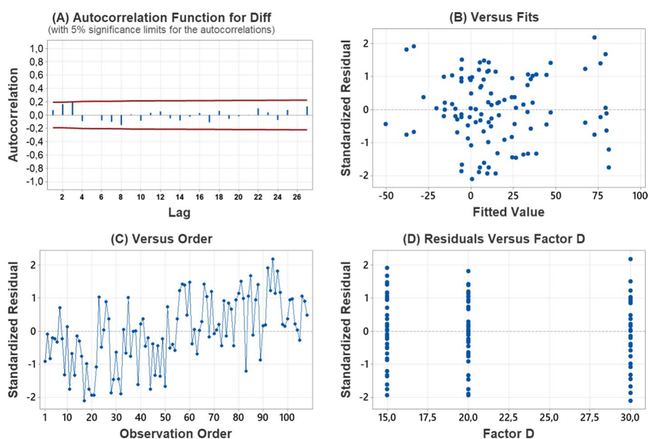
Fig. 4 Validation of assumptions in Software. © 2023 Minitab LLC. A autocorrelation. B residuals versus fits. C residuals versus order. D residuals versus factor D, N: number of non-missing observations; SD: standard deviation; Diff: difference between the c-rtCGM system and FSL
