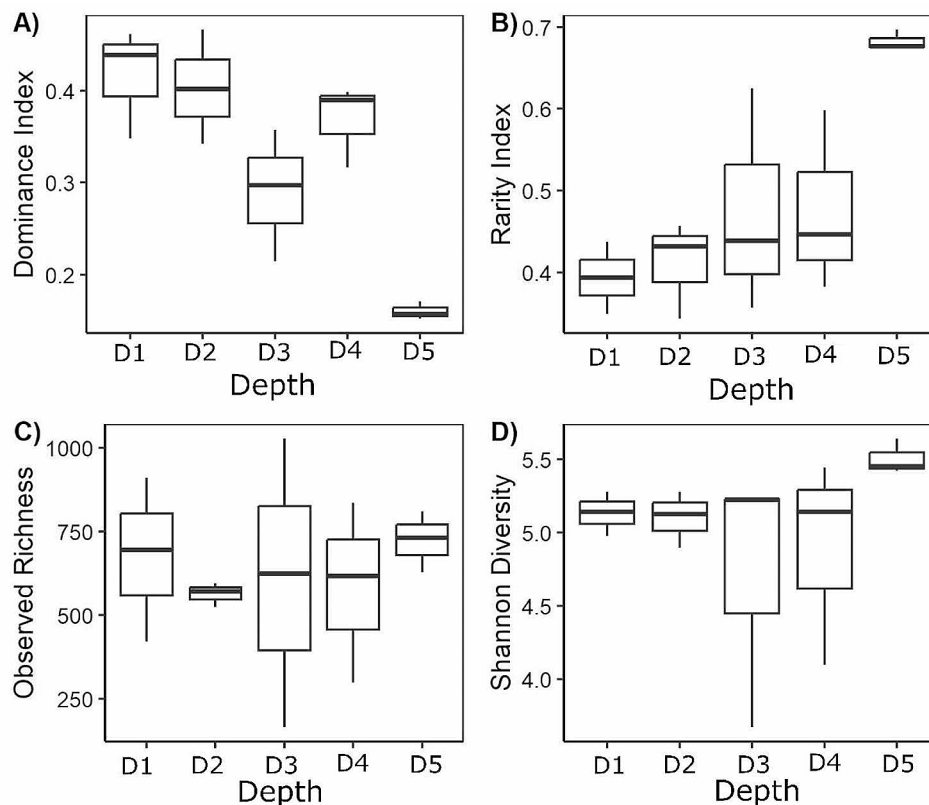
Fig. 4 Comparison of dinoflagellate assemblage alpha diversity at depth zones (D1: 5–10 m, D2: 20–30 m, D3: 45–60 m, D4: 95–120 m, D5: 130–150 m) at Station A, B, and C. (A) Dominance Index, (B) Rarity Index, (C) Observed Richness, and (D) Shannon Diversity. Box boundaries are the interquartile range (IQR); whiskers 1.5 times the IQR; mid-line inside the box is the median. Data from the three stations are combined because PERMANOVA showed no significant differences among stations for any of these indices. Significant differences among different depths are indicated by different lower-case letters
