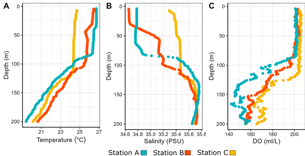
Fig. 5 Conductivity-temperature-depth (CTD) profile data for each station: (A) temperature, (B) salinity, and (C) dissolved oxygen (DO). Colours indicate stations: Station A is blue, Station B is orange, and Station C is yellow. Data from 0 to 200 m below sea surface
