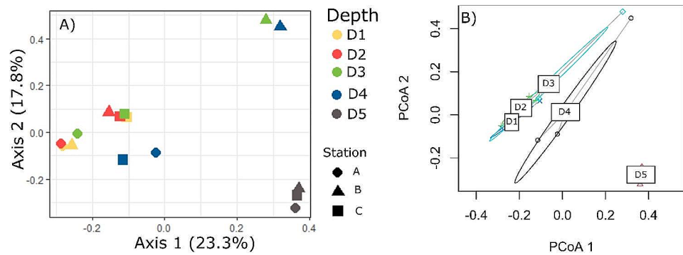
Fig. 3 Ordination plots of Principal Coordinate Analysis (PCoA): (A) ASV abundance among depth zones (D1: 5–10 m, D2: 20–30 m, D3: 45–60 m, D4: 95–120 m, D5: 130–150 m) and stations (Station A, B, and C), and (B) multivariate homogeneity of group dispersions by depth, calculated on Bray-Curtis dissimilarity of normalized Hellinger-transformed ASV abundance data
