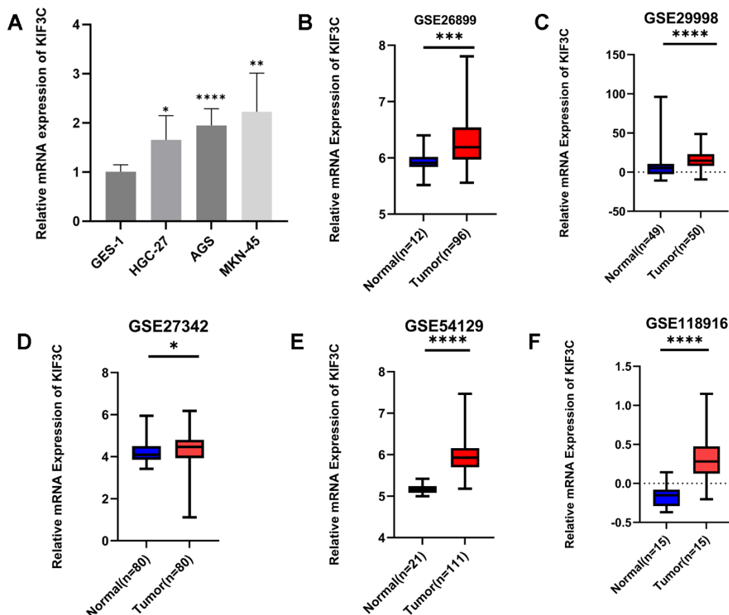
Figure 9. Validation of KIF3C expression. (A) qRT-PCR analysis of KIF3C mRNA in the GC cell lines and normal gastric cell line. KIF3C mRNA levels in GC tissues and normal tissues in (B) GSE26899, (C) GSE29998, (D) GSE27342, (E) GSE54129, (F) GSE118916. *p < 0.05, **p < 0.01, ***p < 0.001, ****p < 0.0001.
