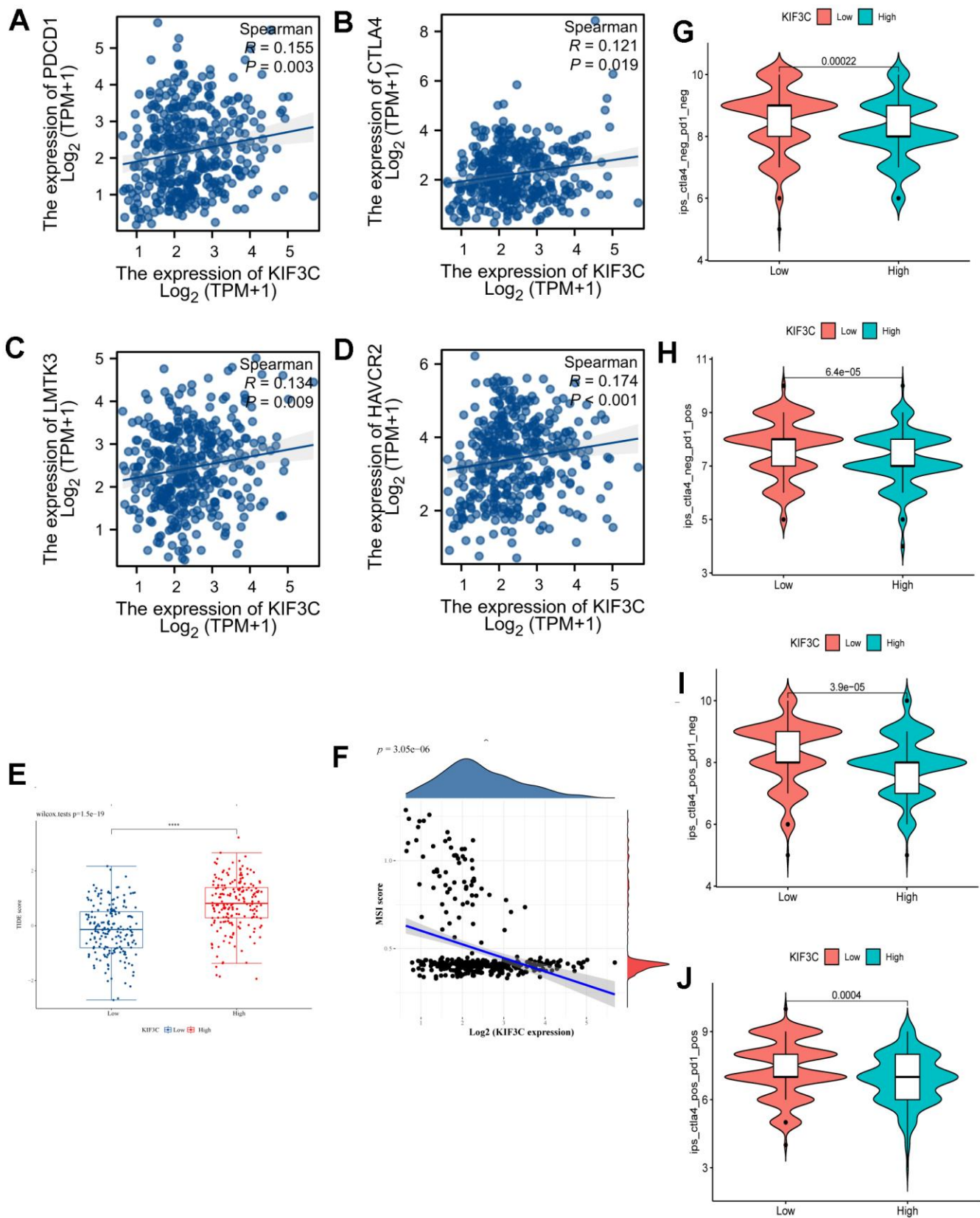
Figure 7. Correlation analysis of KIF3C to the immune checkpoint, TIDE score, MSI, and IPS. (A) PD-1, (B) CTLA4, (C) LMTK3, (D) HAVCR2. (E) TIDE score between KIF3C high- and low-expression expression groups. (F) MSI Score. (G) The IPS, (H) IPS-PD-1/PD-L1/PD-L2, (I) IPS-CTLA4, and (J) IPS-PD-1/PD-L1/PD-L2 + CTLA4.
