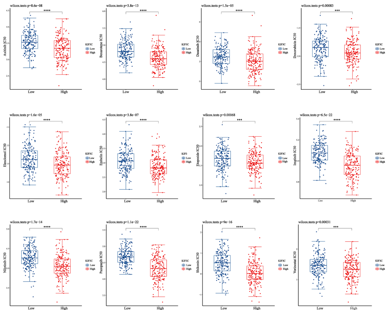
Figure 8. Correction between KIF3C expression and drug sensitivity in gastric cancer. * p < 0.05 ; ** p < 0.01 ; *** p < 0.001 .
