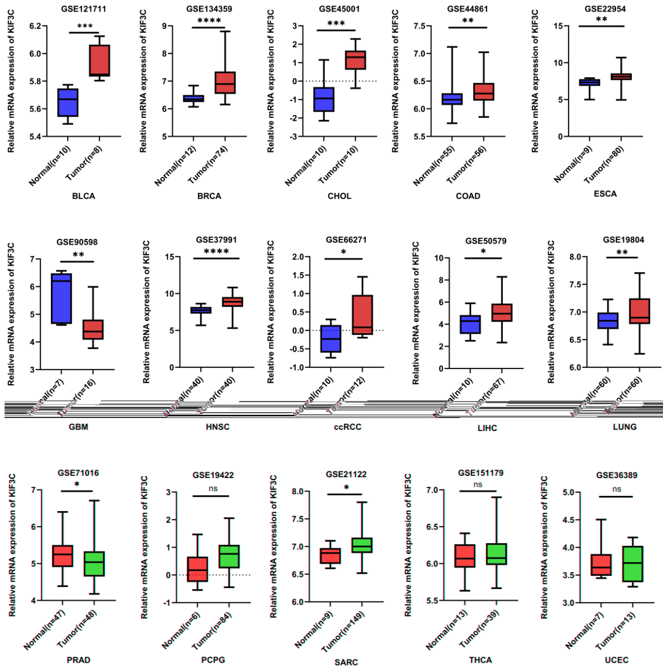
Supplementary Figure 1. The box plots of KIF3C expression levels in GEO.
