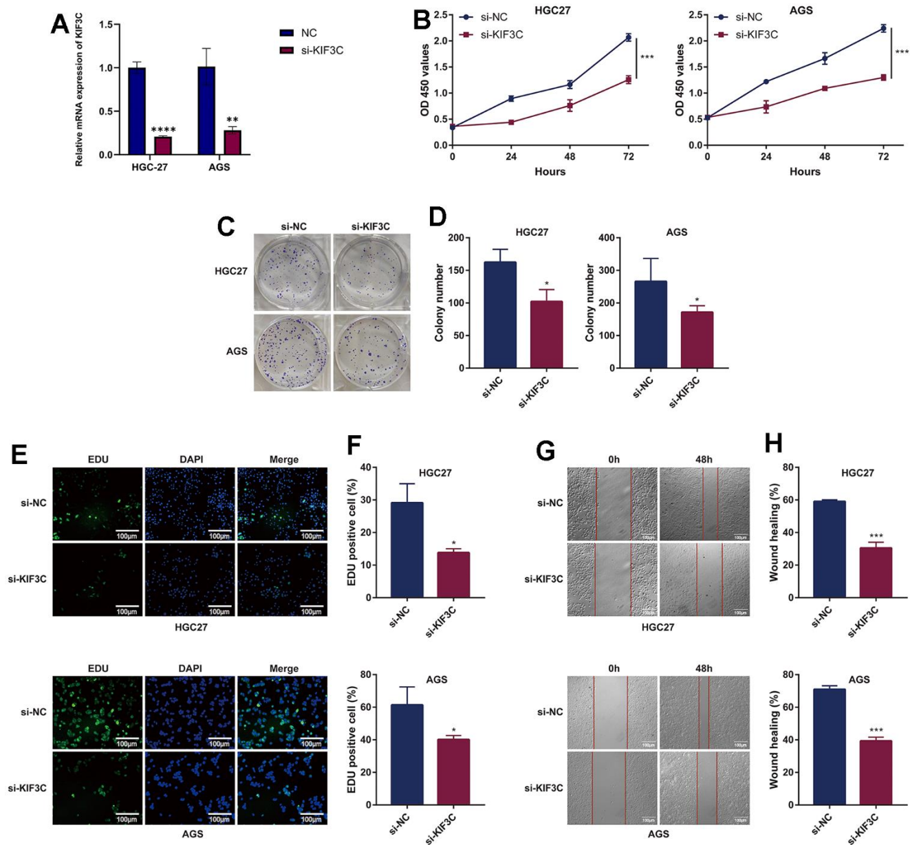
Figure 10. KIF3C knockdown suppresses the malignant phenotype of GC cells. (A) Knockdown efficiency of KIF3C in two Gastric cancer cell lines HGC-27 and AGS, including the si-NC and si-KIF3C groups. (B) CCK-8 assays were applied to detect the effect of KIF3C knockdown on the proliferation of HGC-27 and AGS cell lines. (C) Images of colony formation assay results after KIF3C knockdown in the HGC-27 and AGS cell lines. (D) Representative statistical analysis of the colony formation assay results. (E) DNA replication activity was assessed by an EdU-staining assay (green indicates the EdU-incorporated cells, blue indicates nuclei). GAPDH was used as an internal control. (F) Representative statistical analysis of the EdU assays results. (G) Wound-healing assays employed to detect the migration ability of KIF3C knockdown cells, including HGC-27 and AGS cells. (H) Representative statistical analysis of the wound-healing assays results. * p < 0.05 ; ** p < 0.01 ; *** p < 0.001 .
