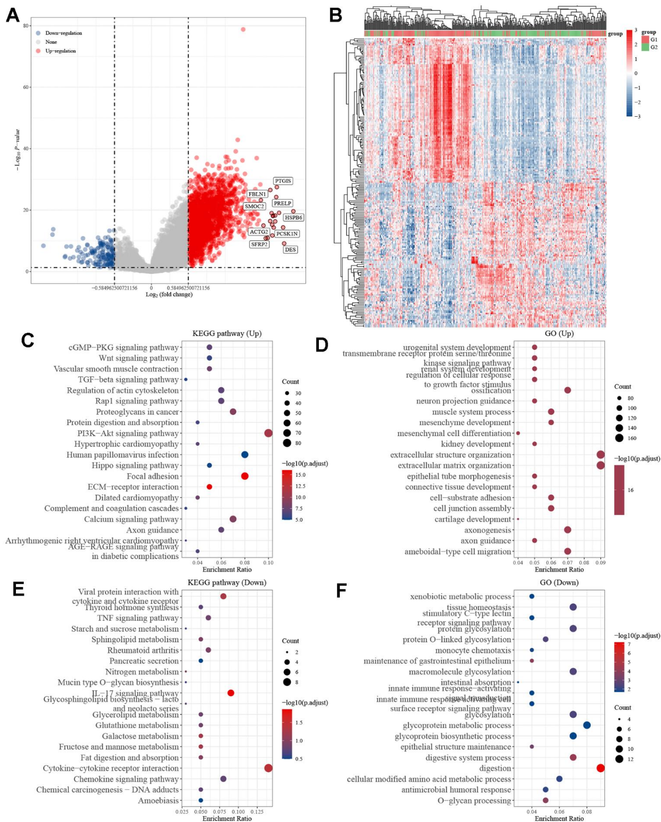
Figure 5. Differentially expressed genes in STAD tissues with high and low KIF3C expression. (A) Volcano map of differentially expressed genes. (B) Heatmap of differentially expressed genes. (C) KEGG and (D) GO enrichment analysis of differentially up-regulated genes. (E) KEGG and (F) GO enrichment analysis of differentially down-regulated genes.
